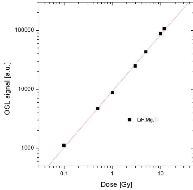
Fig. 2. OSL Dose–response curve for the LiF:Mg,Ti dosimeters.
