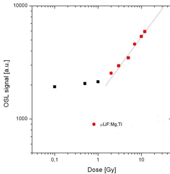
Fig. 3. OSL Dose–response curve for the microLiF:Mg,Ti TL dosimeters.
