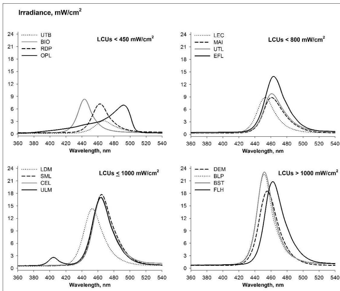
Figure 1. Spectral emission of the light-curing units (LCUs) tested: Ultra Blue IV Plus (UTB), Biolux (BIO), Radii Plus (RDP), Optilux 501-QTH (OPL), LEC 470 II (LEC), Mais (MAI), UltraLight III (UTL), Elipar Freelight 2 (EFL), LEDemetron (LDM), Smart Lite PS (SML), Celalux (CEL), Ultra-Lume LED 5 (ULM), Demi (DEM), Bluephase (BLP), Blue Star I (BST), and FLASHlite 1401 (FLH).
