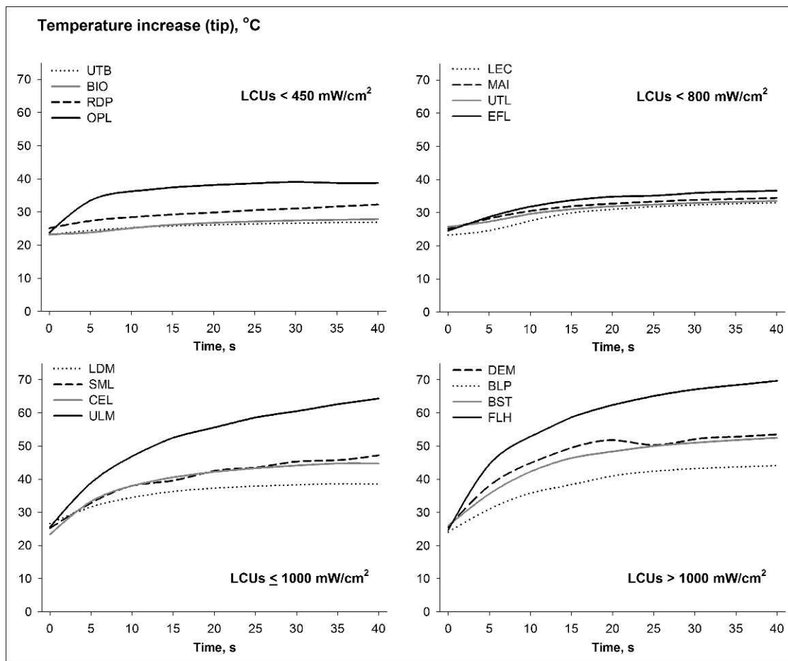
Figure 2. Profiles of temperature increase at the light guide tip over the 40-second exposure time. The temperature increase followed a logarithmic growth pattern for the LCUs with irradiance \geq 1000 \text{ mW/cm}^2 .
