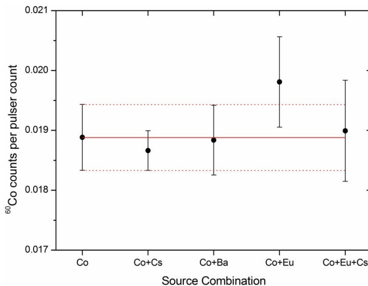
Figure 4: Pulser-corrected count rates observed for the same ^{60}\text{Co} source under different radioactive source combinations – the red lines represent the results obtained without any additional sources (full line) and its 1\text{-}\sigma uncertainty (dotted lines).
