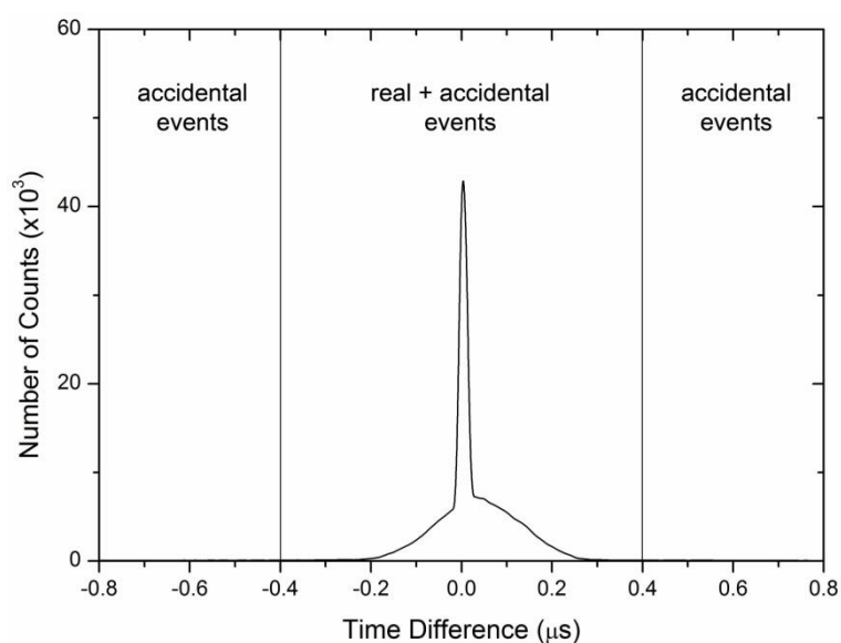
Figure 1: Typical time spectrum from the coincidence system showing the regions where the events can be considered 100% accidental and the region where there are both real and accidental events – the narrow peak originates from the pulser, whereas the wider one is from the detector events.
