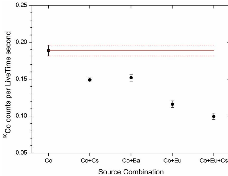
Figure 3: Count rates observed for the same ^{60}\text{Co} source under different radioactive source combinations – the red lines represent the results obtained without any additional sources (full line) and its 1\text{-}\sigma uncertainty (dotted lines).
