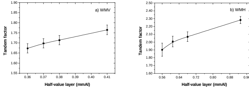
Fig. 6. Tandem curves for (a) WMV and (b) WMH radiation qualities
