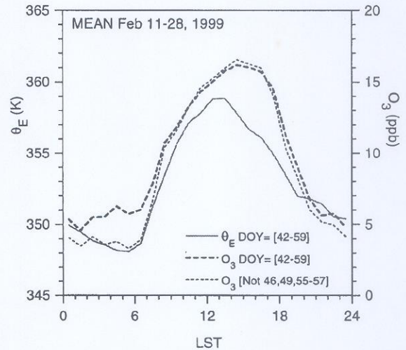
Figure 1. Mean diurnal cycle of \theta_E and \text{O}_3 at surface from 11 to 28 February 1999.
