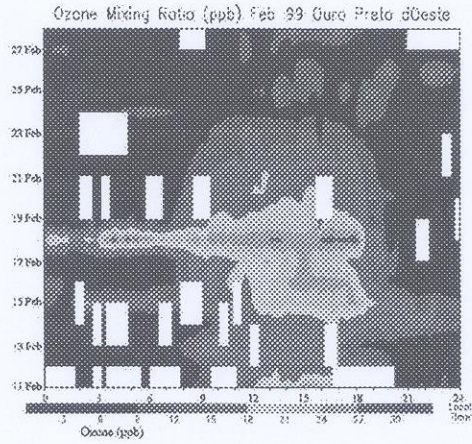
Figure 2. Ozone distributions in Rondônia from 11 to 28 February 1999.
