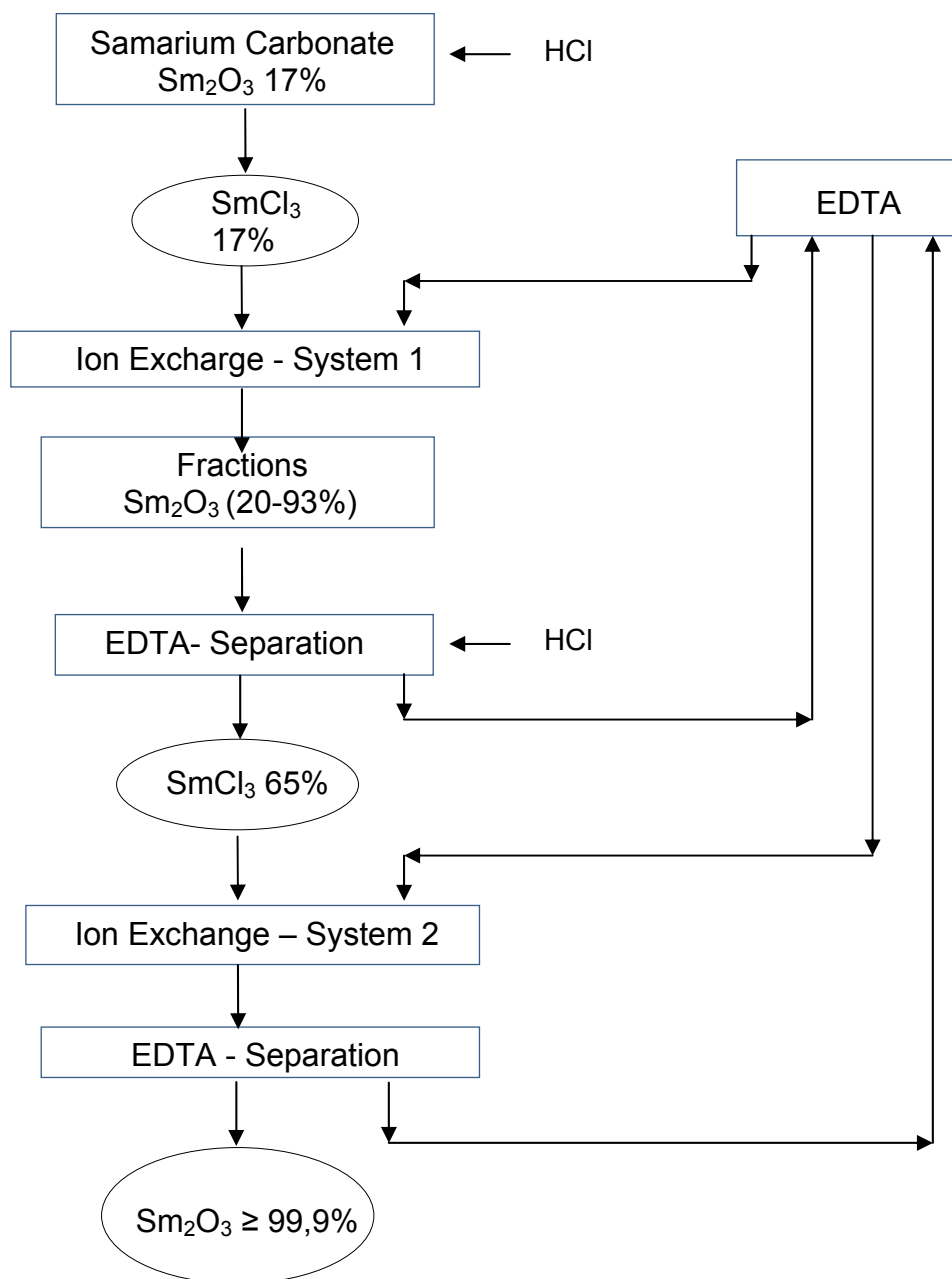
Figure 1: Procedure for the preparation of pure samarium acetates for use in P&D at IPEN- CNEN/SP
