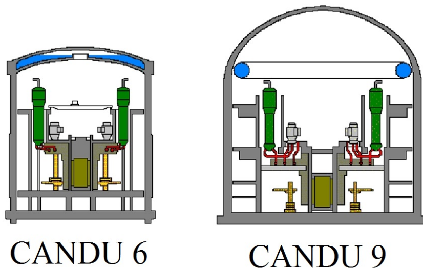
Figure 5: CANDU 6 and CANDU 9 reactor building layout [27].
