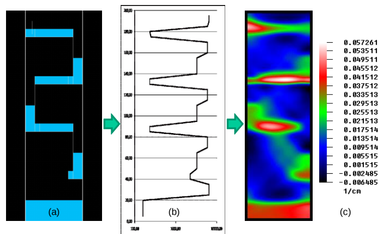
Figure 2. Computed simulated column arrangement (a), resulting gamma ray profile (b) and reconstructed tomographic image of a trayed column (c).
