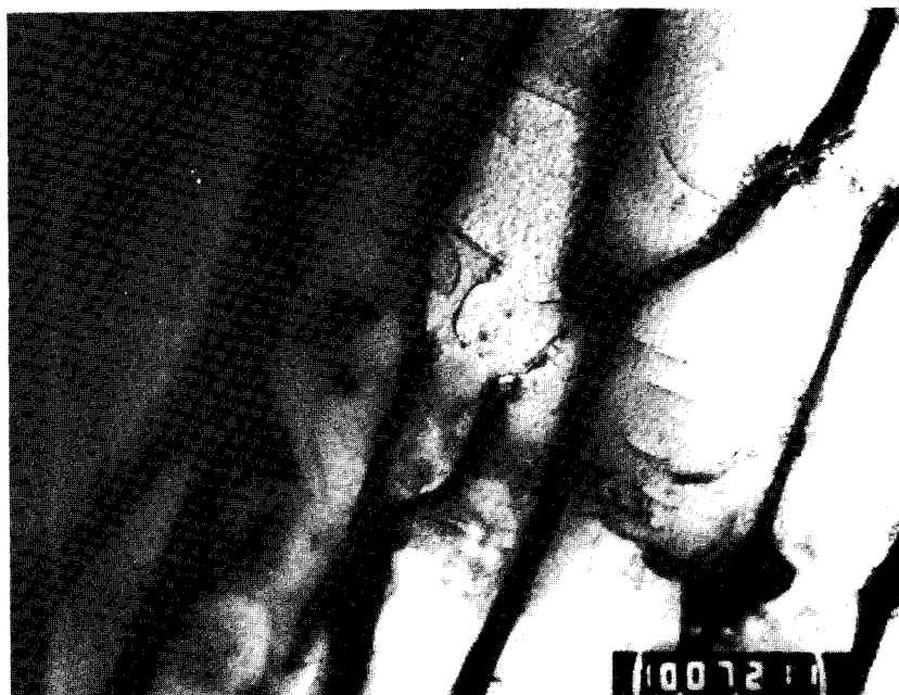
FIGURE 9. Transmission electron micrograph of Zr-2.5wt%Nb alloy tempered at 600°C for 1000 hours (15,000X).
