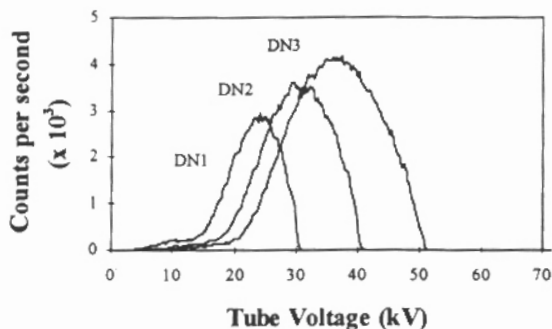
Figure 1. The maximum tube voltage (kVp) determination to DN1, DN2 and DN3 qualities.
