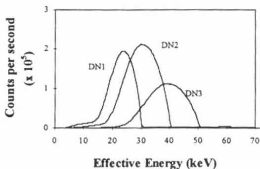
Figure 2. Spectra of the qualities DN1, DN2 and DN3.
