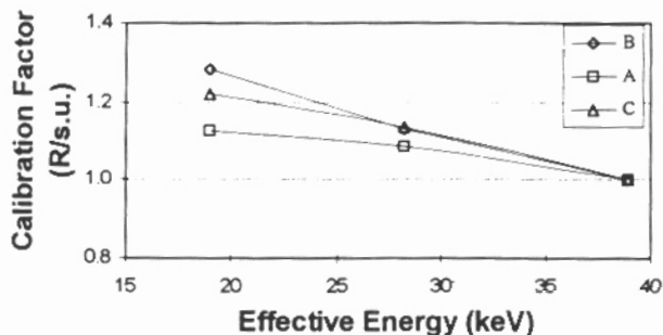
Figure 3. Energy Dependence of the IPEN parallel plate ionization chambers. All values were normalized to 50 kV to make easy the comparison.
