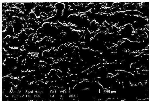
Fig. 1. SEM of 304L SS filter used in this investigation.
