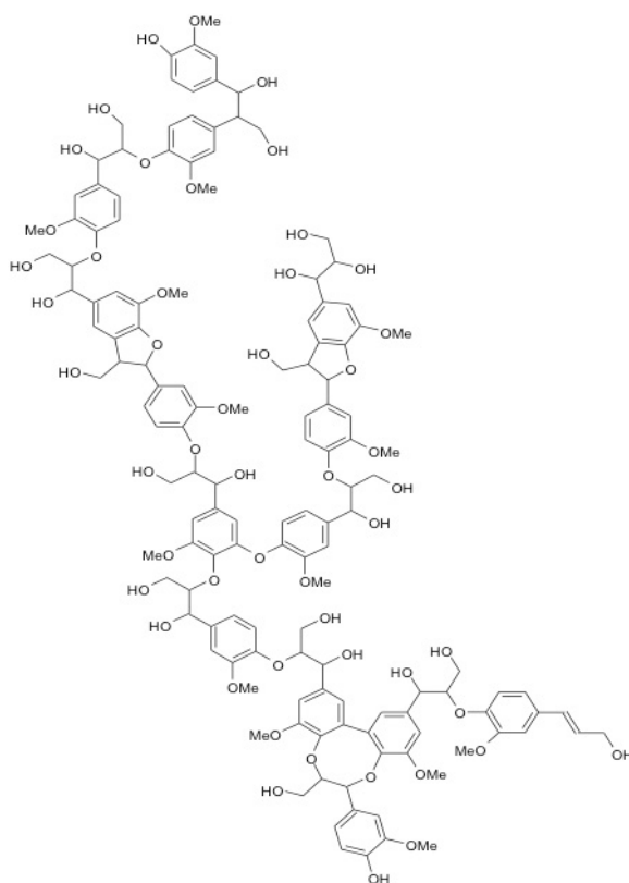
FIG. 15.8. Diagram of the structure of lignin [15.21].
