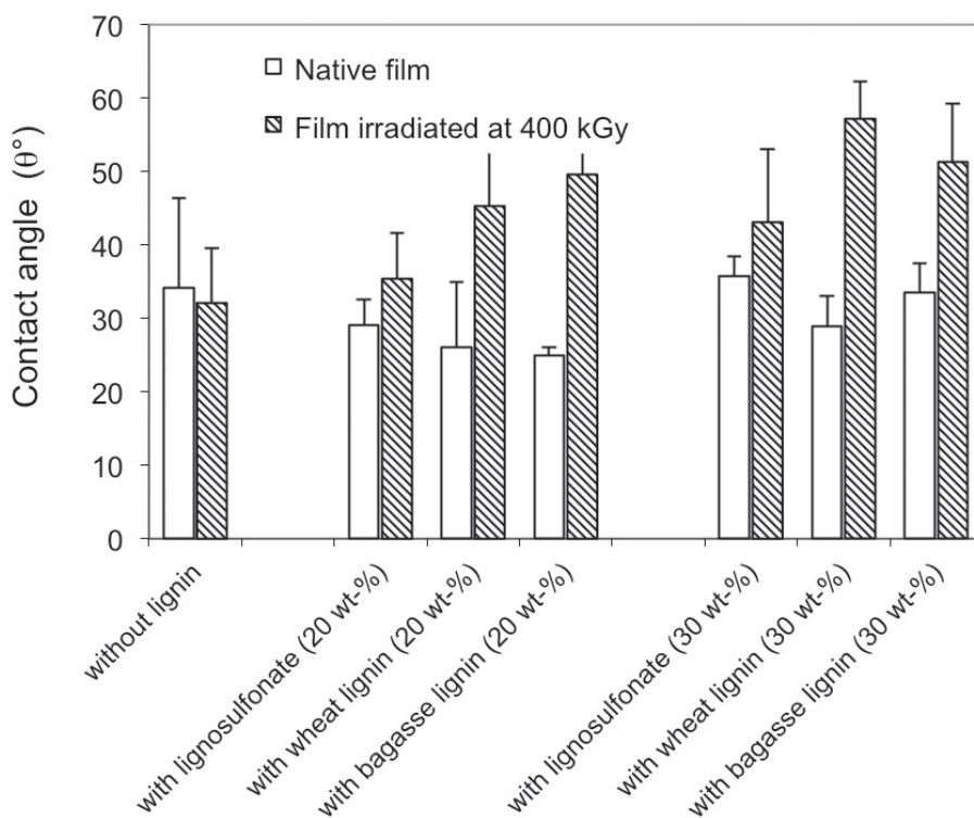
FIG. 15.9. Effects of the presence of lignin and EB irradiation on the contact angle of a water droplet on starch based films.
