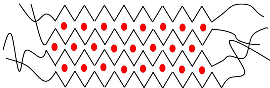
FIG. 2.6. Egg box model proposed for the interaction between polyuronates and \text{Ca}^{2+} ions (denoted as red circles between two polymeric chains).
