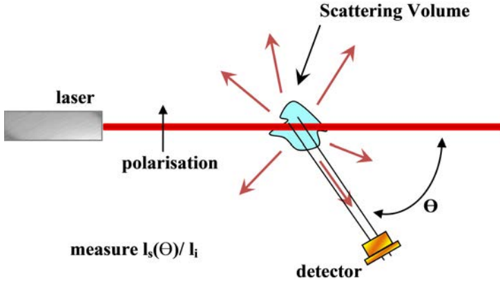
FIG. 6.3. The path of light scattered through a polymer solution. Reproduced with permission from Wyatt Technology.
