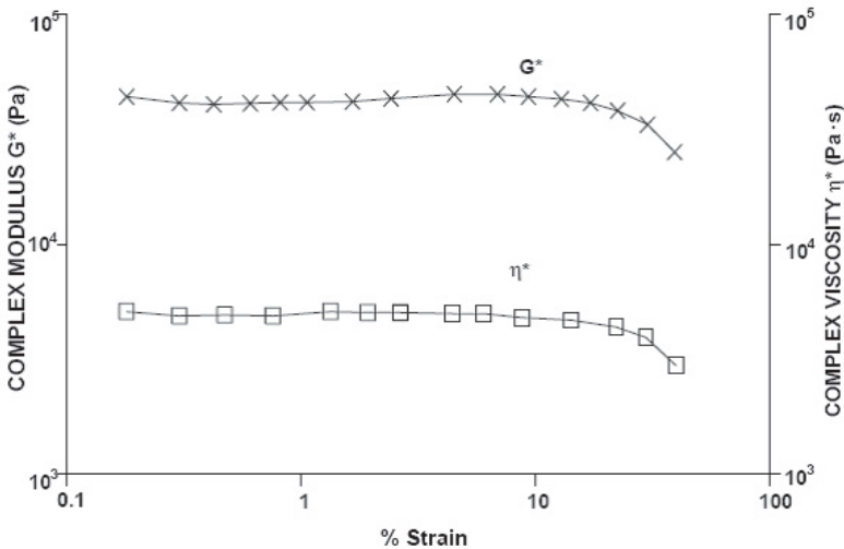
FIG. 6.22. Amplitude sweep curve for determining linear viscoelastic region.
