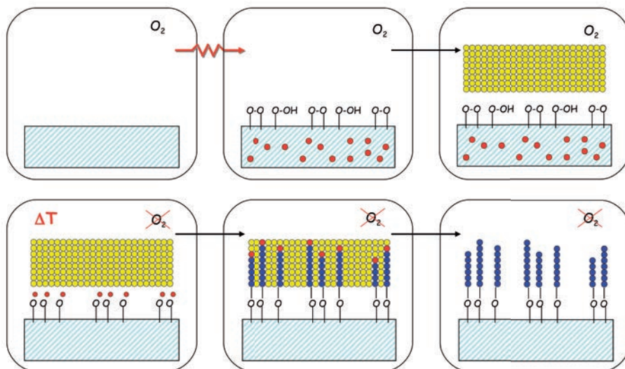
FIG. 3.15. A scheme of pre-irradiation grafting (irradiation in the presence of oxygen). Red dots denote radicals, yellow dots — monomer molecules, blue dots — monomer molecules incorporated in the grafted chains.
