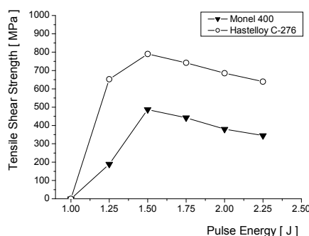
Figure 11. Relationship between pulse energy and tensile shear strength.
