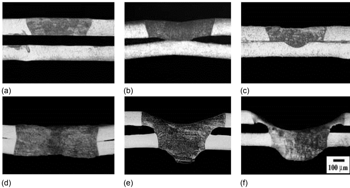
Figure 7. Cross sections of Hastelloy C-276 lap joints made with pulsed Nd:YAG laser welding with different pulse energies ( E_p ): a) 1.0 J, b) 1.25 J, c) 1.50 J, d) 1.75 J, e) 2.0 J and f) 2.25 J. All figures have the same magnification as shown in (f).
