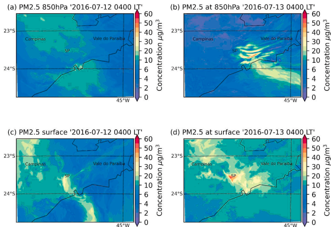
Fig. 6. PM2.5 concentrations simulated by EURAD-IM on the 1-km resolution grid at 850 hPa, 0400 LT for (a) PM2.5 on July 12; (b) PM2.5 on July 13 and at surface for (c) PM2.5 on July 12; (d) PM2.5 on July 13, 2016.
