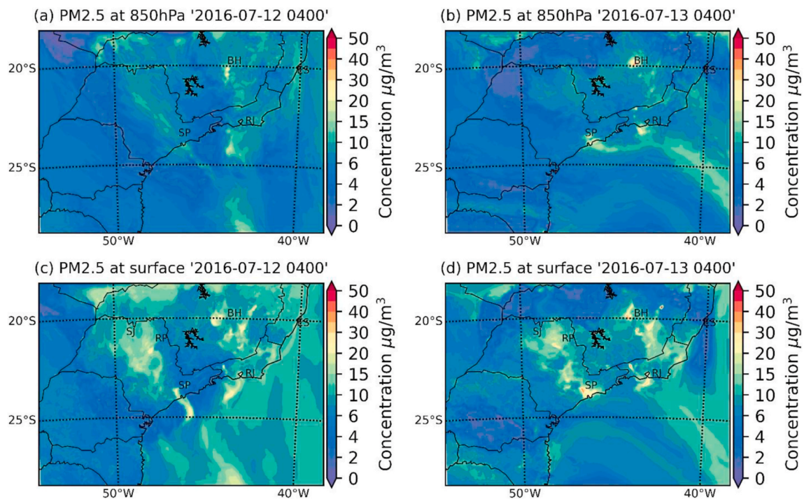
Fig. 5. PM2.5 concentration simulated by EURAD-IM with 5-km horizontal resolution at 0400 LT at 850 hPa on July 12 (a), and July 13(b) (top panels), and at surface on July 12 (c), and July 13 (d) (bottom panels).
