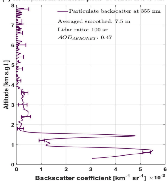
Fig. 9. AOD from Terra (MOD04_L2), Aqua (MYD04_L2), MODIS Fire hotspots and Thermal Anomalies product from Terra (MOD14), Aqua (MYD14) across Brazil and other South American countries (a) on October 24, 2016 and (b) on October 25, 2016 (Source: Nasa, 2020); the Backscatter backscatter profiles on October 24, 2016, between 10:30 and 11:30 LT from the IPEN Lidar in the MASP at: (c) 355 and (d) 532 nm.
