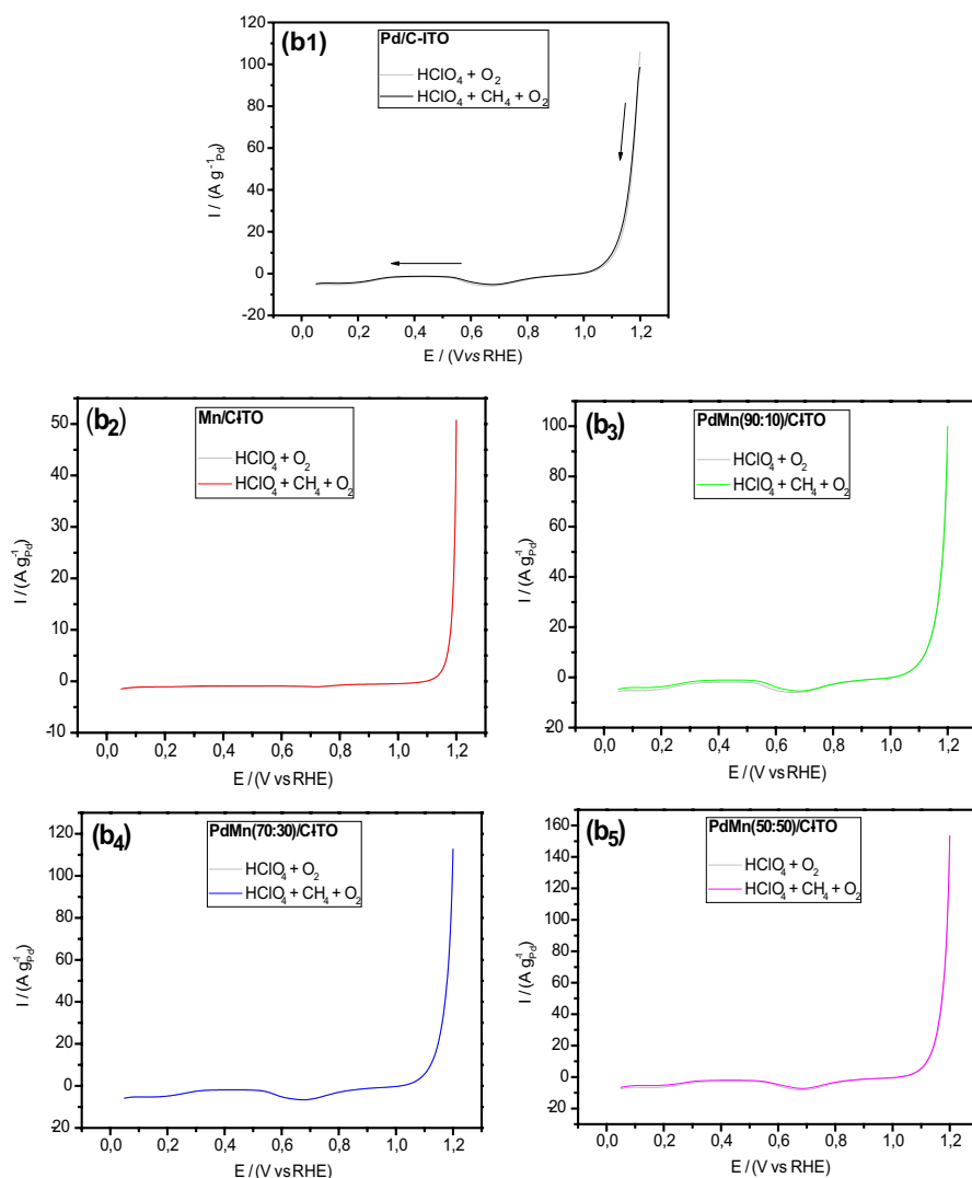
Fig. 7 Linear sweep voltammetry for b 1 Pd/C-ITO, b 2 Mn/C-ITO, b 3 PdMn(90:10)/C-ITO, b 4 PdMn(70:30)/C-ITO and b 5 PdMn(50:50)/C-ITO in O 2 purged in 0.5 mol L -1 HClO 4 electrolyte and in (O 2 + CH 4 ) gases purged in 0.5 mol L -1 HClO 4 electrolyte at room temperature at a scan rate of 10 mV s -1 in anodic potential sweeps from 1.2 to 0.05 V versus RHE
