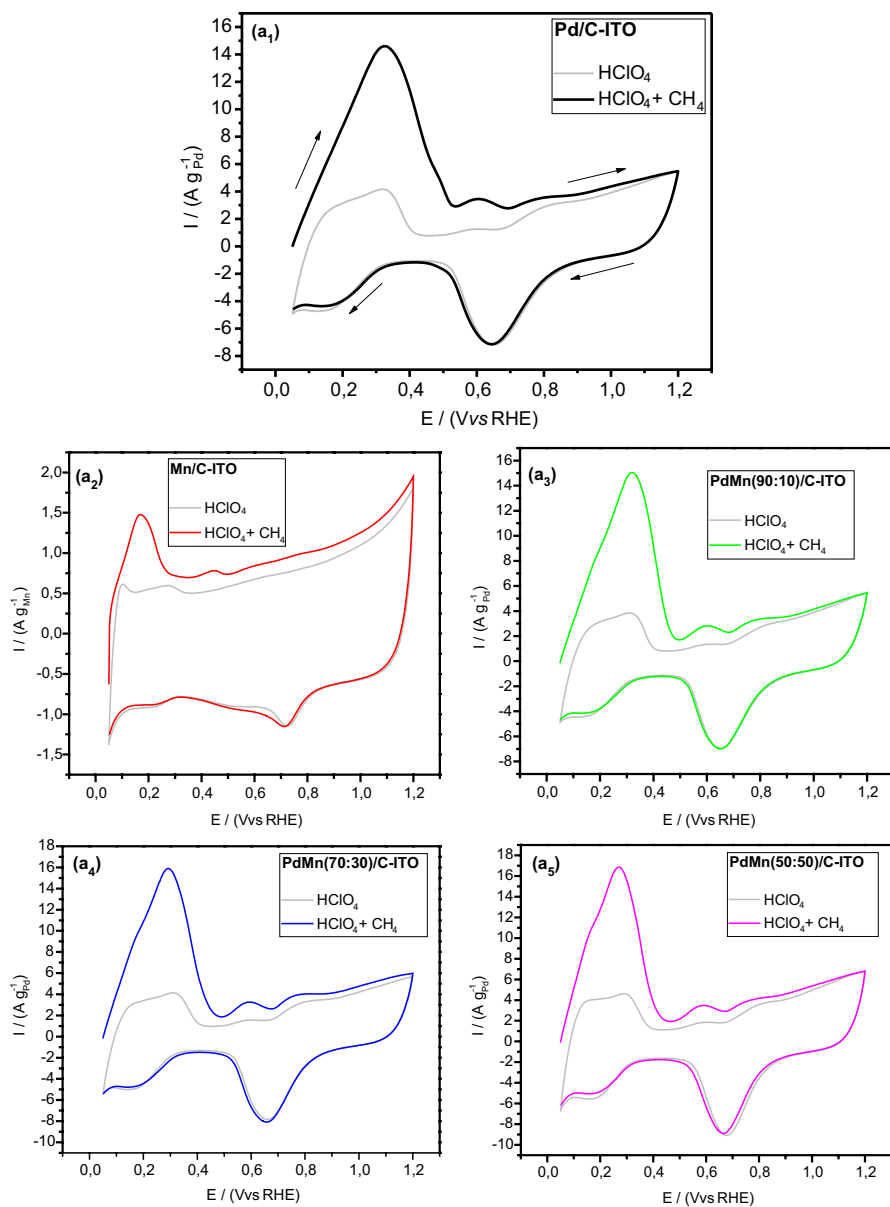
Fig. 6 Comparison of the voltammograms for a 1 Pd/C-ITO, a 2 Mn/C-ITO, a 3 PdMn(90:10)/C-ITO, a 4 PdMn(70:30)/C-ITO and a 5 PdMn(50:50)/C-ITO: in a 0.5 \text{ mol L}^{-1} \text{ HClO}_4 electrolyte and 0.5 \text{ mol L}^{-1} \text{ HClO}_4 electrolyte + \text{CH}_4 gas, \nu = 10 \text{ mV s}^{-1} ; ambient temperature (300 K)
