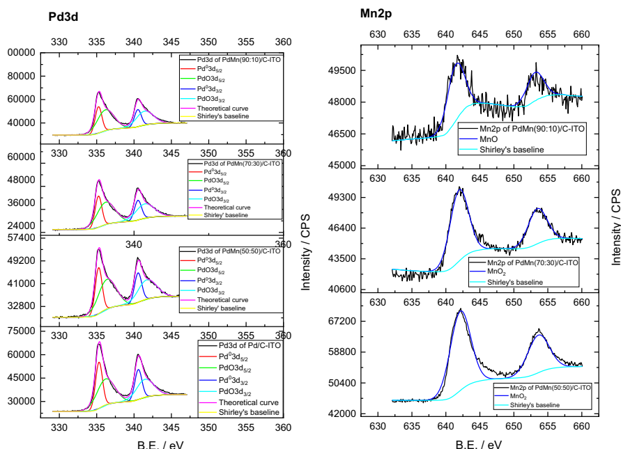
Fig. 5 XPS spectra of Pd3d and Mn2p of Pd/C-ITO, PdMn(90:10)/C-ITO, PdMn(70:30)/C-ITO and PdMn(50:50)/C-ITO electrocatalysts
