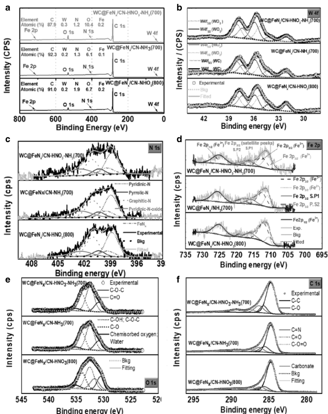
Fig. 5 X-ray photoelectron spectroscopy (XPS) spectra of the WC@-FeN x /CN-HNO 3 (800), WC@-FeN x /CN-NH 3 (700), and WC@-FeN x /CN-HNO 3 -NH 3 (700) electrocatalysts. a Wide scan spectrum. b High-resolution W 4f spectrum with peaks deconvoluted into WC, WO 2 , and WO 3 . c High-resolution N 1s spectrum with the peaks deconvoluted into
