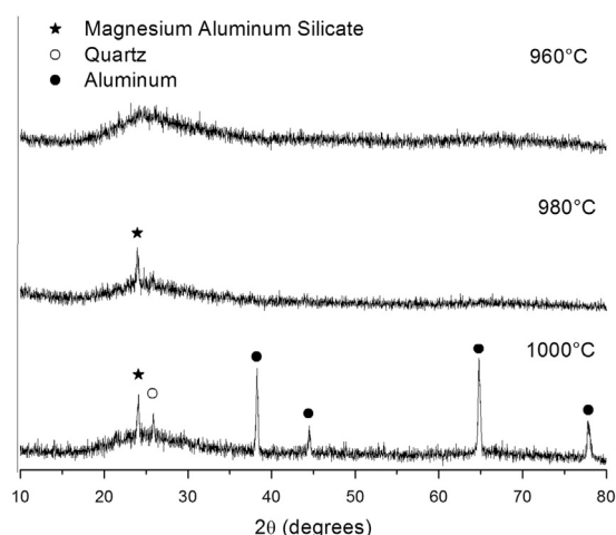
Fig. 9. X-ray diffraction patterns of pellets treated at 960 °C, 980 °C, and 1000 °C.
