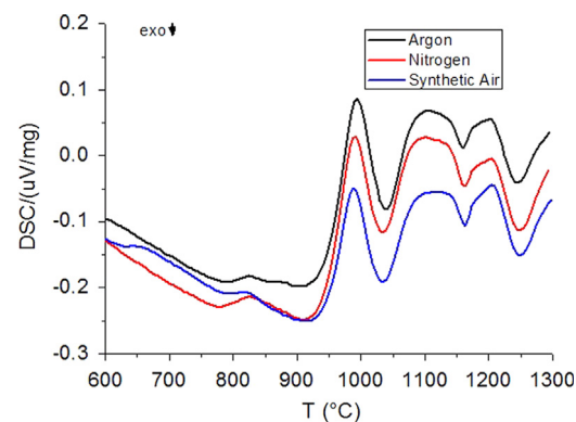
Fig. 5. DSC curves of glass powder. Analyses were performed on dynamic atmospheres of synthetic air, argon, and nitrogen. The heating rate was 10 °C/min in alumina sample holders.
