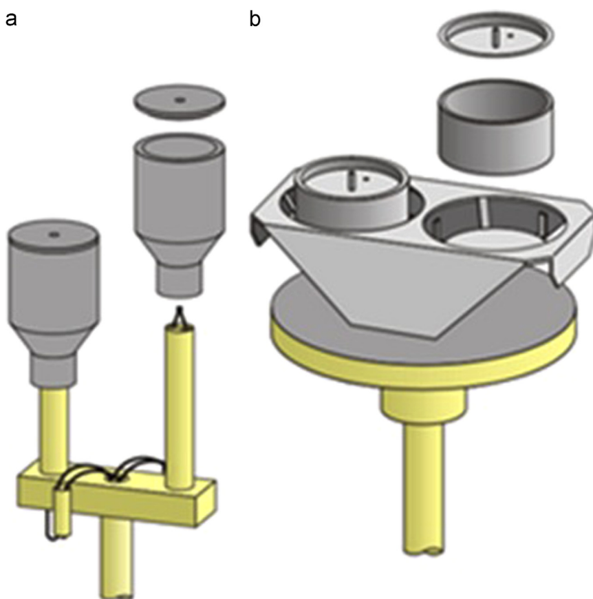
Fig. 3. Measurement assembly: (a) DTA and (b) DSC [11].
