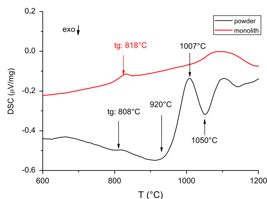
Fig. 1. DSC curves of glass samples as powder and glass monolith. The glass transition temperatures ( T_g ) were determined in the range of 808–820 °C. Analyses were performed on a dynamic synthetic air atmosphere with a heating rate of 10 °C/min in an alumina sample holder.
