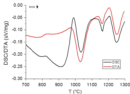
Fig. 4. DSC and DTA curves of glass powder in alumina sample holders. The analyses were performed on a dynamic synthetic air atmosphere with a heating rate of 10 °C/min.
