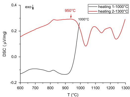
Fig. 7. DSC curves of glass powder in two steps: heated to 1000 °C, cooled to room temperature and reheated to 1300 °C. Analyses were performed on a synthetic air atmosphere, heating rate of 10 °C/min, in an alumina sample holder.
