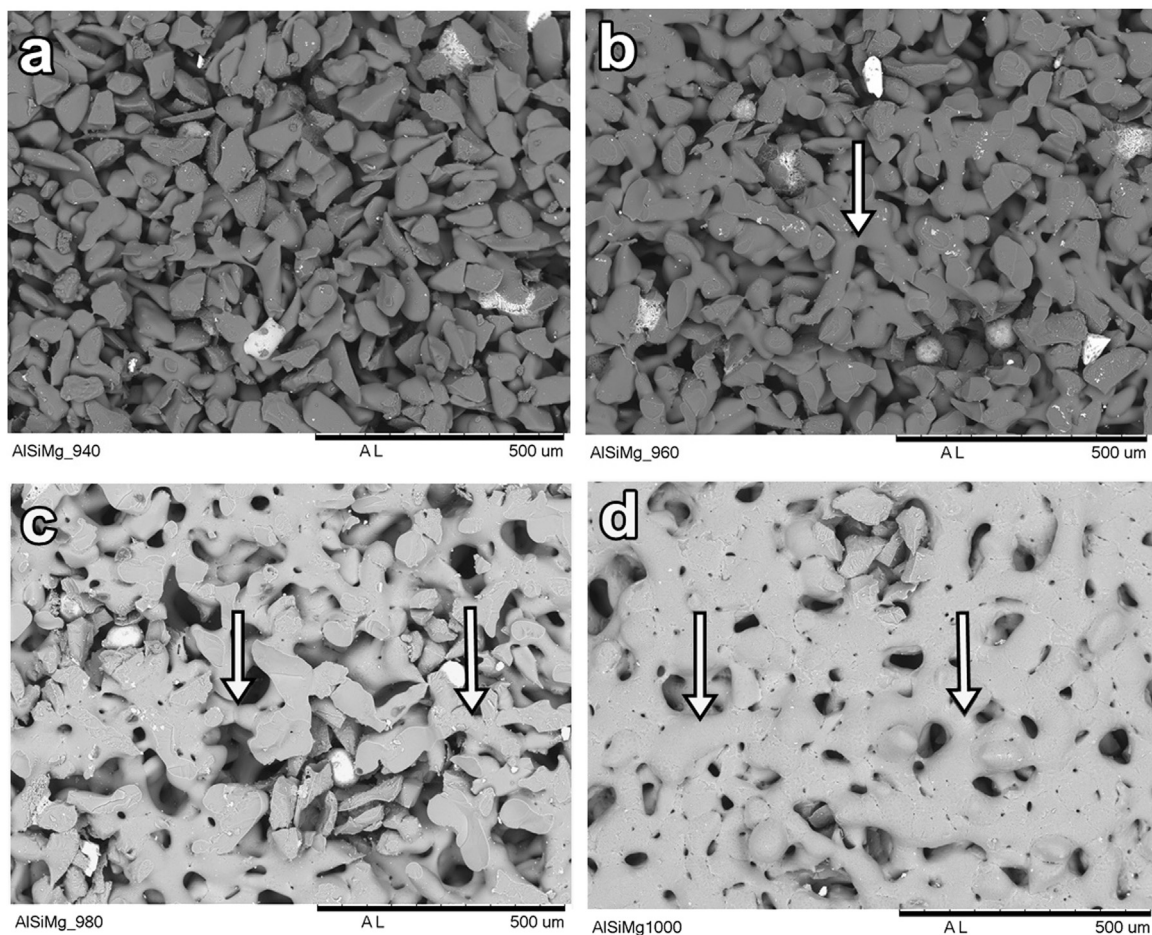
Fig. 8. SEM micrographs of the pellets treated at (a) 940 °C, (b) 960 °C, (c) 980 °C, and (d) 1000 °C. The arrows indicate the formation of necks between particles.
