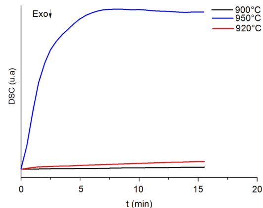
Fig. 6. Isothermal DSC curves. Analyses were performed in synthetic air atmosphere, in alumina sample holders, at 900 °C, 920 °C, and 950 °C.
