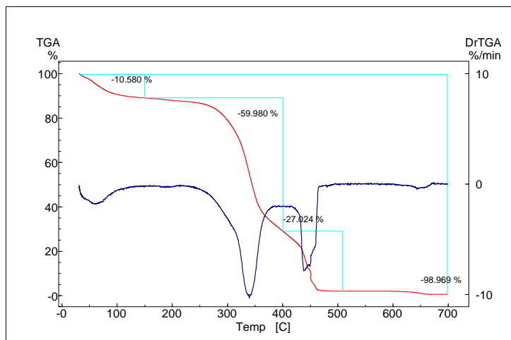
Figure 5. TG/DTG curve for 25kGy-irradiated cedro-rosa .
