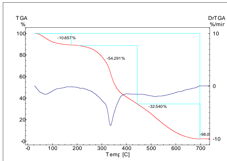
Figure 1. TG/DTG curve for non-irradiated Imbuia .
