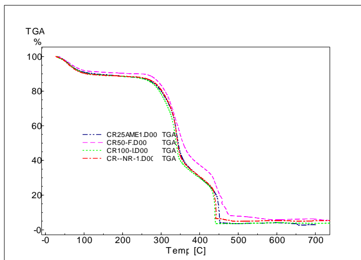
Figure 6. TG curves for non-irradiated, 25kGy-, 50kGy-, 100kGy-irradiated cedro-rosa .
