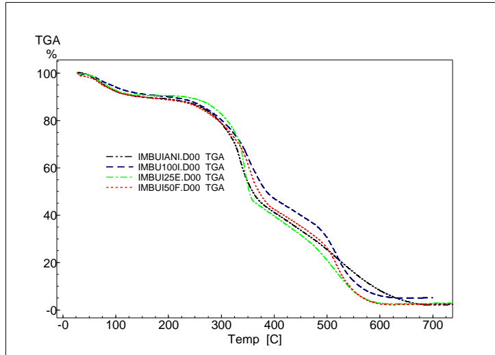
Figure 3. TG curves for non-irradiated, 25kGy-, 50kGy-, 100kGy-irradiated Imbuia .
