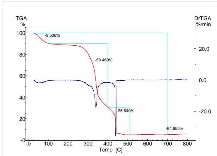
Figure 4. TG/DTG curve for non-irradiated cedro-rosa .
