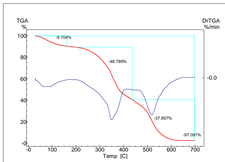
Figure 2. TG/DTG curve for 100kGy-irradiated Imbuia .
