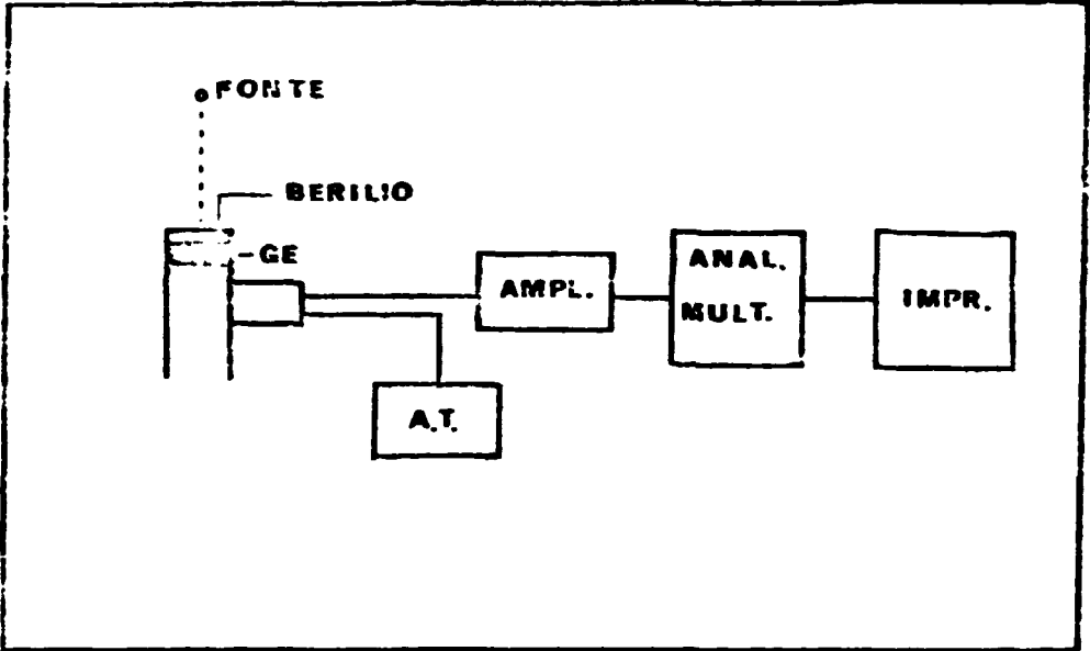
ARRANJO EXPERIMENTAL
