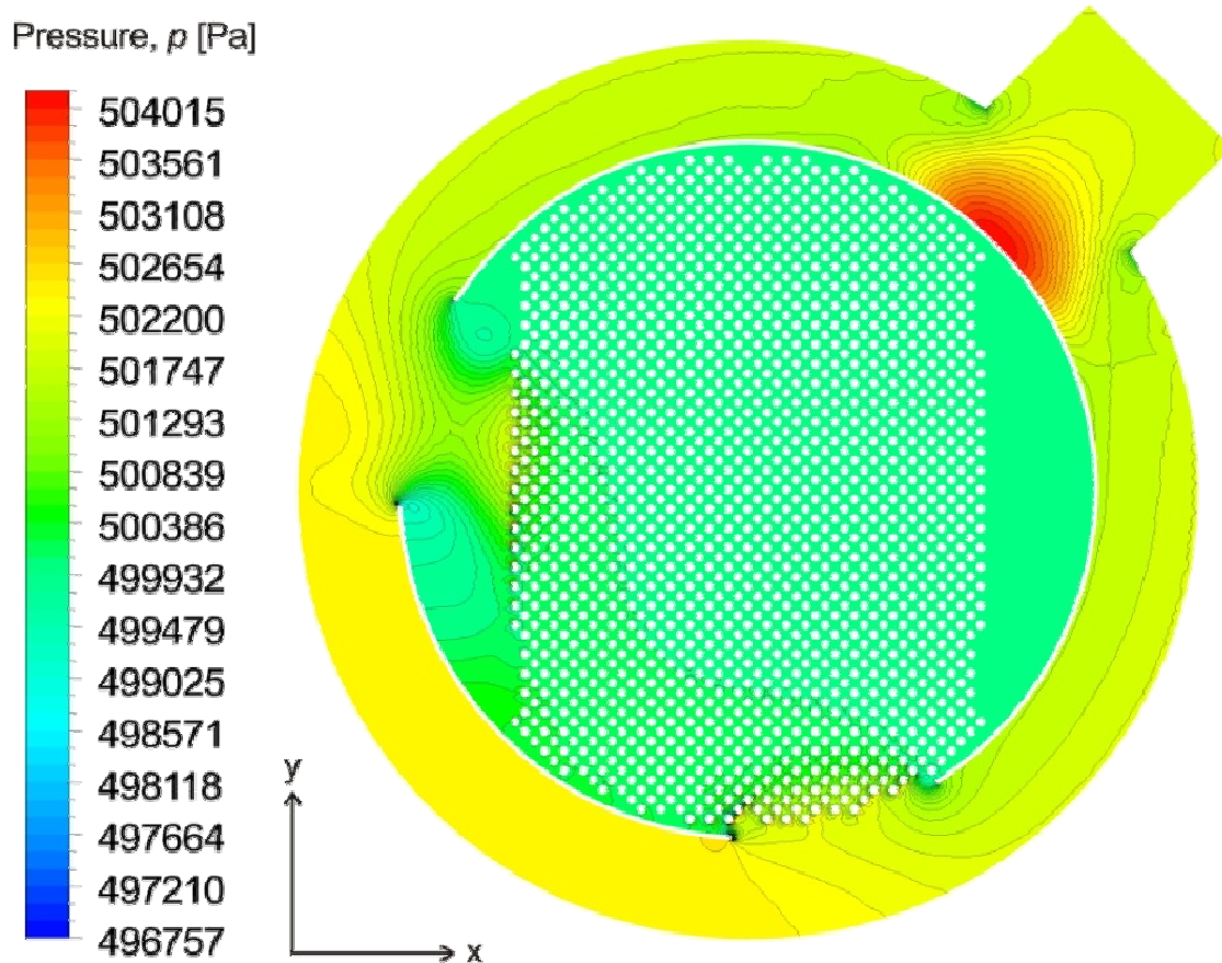
Figure 4. Pressure contour - section AA.
