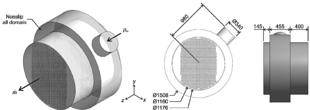
Figure 2. Tridimensional model, all dimensions in millimeters.
