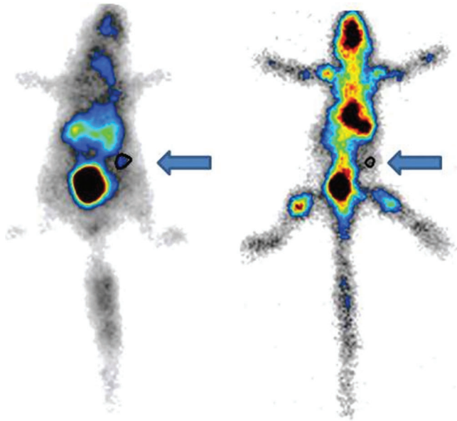
Figure 8 - Gamma camera imaging of the femur graft after 15 days of abdominal storage. Left side ( ^{99m}\text{Tc} -HYNIC-E-[c(RGDfK) 2 ] region of interest (ROI= 0.5%) and right side ^{99m}\text{Tc} -MDP uptake (ROI= 0.10%). The arrows indicate the implanted bone.
