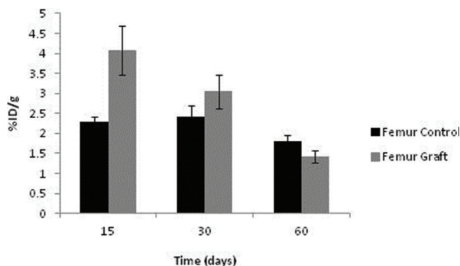
Figure 6 - Uptake of ^{99m}\text{Tc} -HYNIC-E-c(RGDfK) 2 in the femur.
