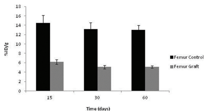
Figure 7 - Uptake of ^{99m}\text{Tc} -MDP in the femur.
