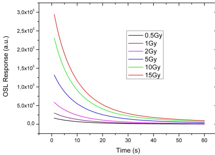
Fig. 3: OSL response curve of LiF:Mg,Ti according to the beta radiation doses of ^{90}\text{Sr}/^{90}\text{Y} .
