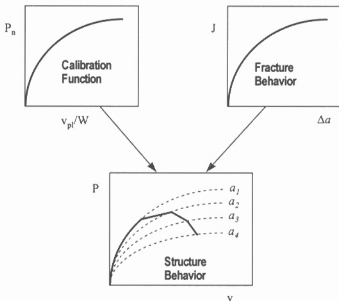
FIG. 1—Schematic of the Ductile Fracture Method
