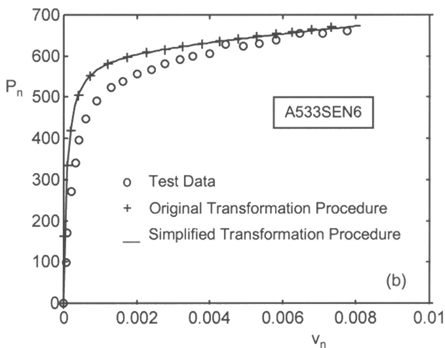
FIG. 4—Calibration curves for the SENT specimens
