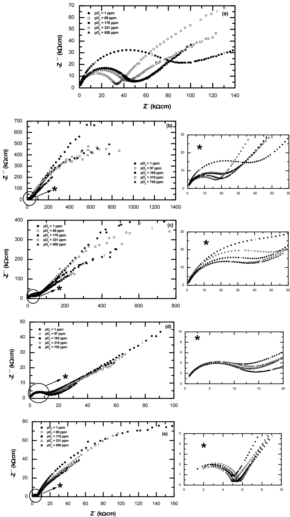
Fig. 5. Impedance diagrams of (\text{ZrO}_2: 8 \text{ mol\% MgO})_x (\text{ZrO}_2: 3 \text{ mol\% Y}_2\text{O}_3)_{1-x} pellets, for x = 1 (a), 0.8 (b), 0.5 (c), 0.2 (d) and 0 (e) at 600^\circ\text{C} as a function of the partial pressure of oxygen from 1 to 850 ppm.
