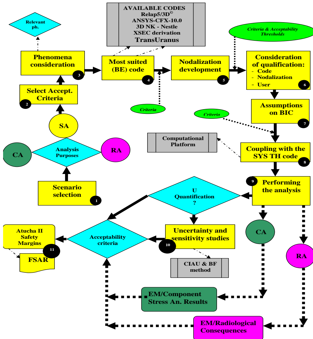
Figure 2: BEPU flow-diagram
