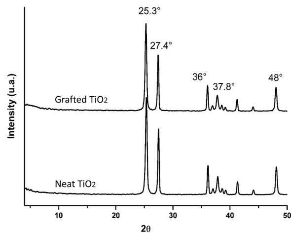
Fig. 2. XRD patterns of neat and grafted with PGMA \text{TiO}_2 .
