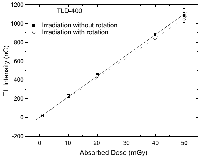
Fig. 2. Calibration curves obtained for different TLDs in the diagnostic radiology standard beam of RQA9, with and without rotation of the pellets.
