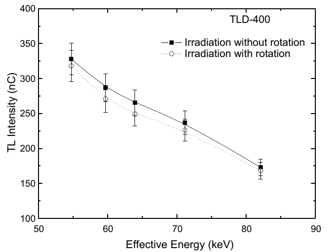
Fig. 3. Energy dependence curves obtained for different TLDs in diagnostic radiology standard beams (absorbed dose of 10 mGy), with and without rotation of the pellets.
