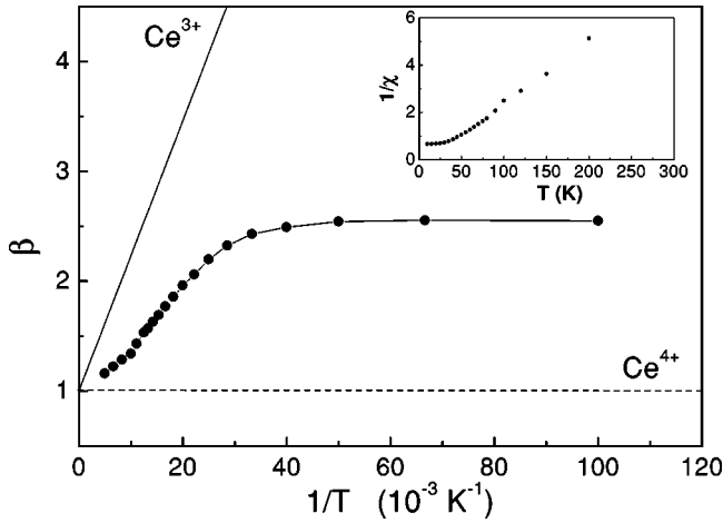
FIG. 7. The local paramagnetic enhancement factor \beta as a function of the inverse of the temperature for ^{140}\text{Ce} at Ce sites in \text{CeMn}_2\text{Ge}_2 . The inset shows the temperature dependence of the inverse of the local susceptibility \chi .
