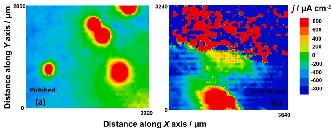
Fig. 13. SVET maps obtained above freely corroding AA2098-T351 surfaces in (a) polished and (b) as-received conditions. They were recorded after approximately 120 min of immersion in 5 mmol L -1 NaCl solution.
