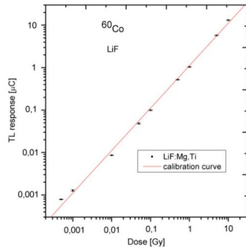
Fig. 3: Dose-response curve of \text{LiF}:\text{Mg,Ti} for irradiation in ^{60}\text{Co} gamma radiation source in air and under electronic equilibrium conditions (PMMA plates).
