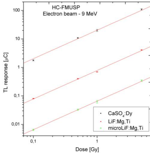
Fig. 6: Dose-response curves to 9 MeV electrons using solid water phantom.
