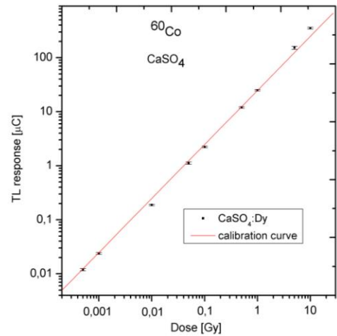
Fig. 2: Dose-response curve of \text{CaSO}_4:\text{Dy} for irradiation in ^{60}\text{Co} gamma radiation source in air and under electronic equilibrium conditions (PMMA plates).
