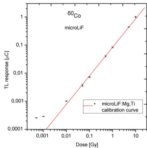
Fig. 4: Dose-response curve of \text{microLiF}:\text{Mg,Ti} for irradiation in ^{60}\text{Co} gamma radiation source in air and under electronic equilibrium conditions (PMMA plates).
