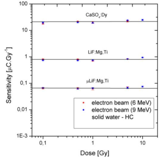
Fig. 7: Average sensitivity of the TLDs to 6 and 9 MeV electrons using solid water phantom.
