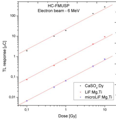
Fig. 5: Dose-response curves to 6 MeV electrons using solid water phantom.
