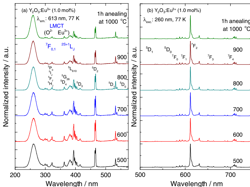
Figure 7. The (a) excitation spectra of \text{Y}_2\text{O}_3:\text{Eu}^{3+} (1.0 mol%), with emission monitored at 613 nm; (b) emission spectra, with excitation at 260 nm, recorded at 77 K.
