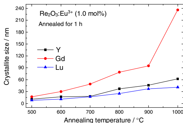
Figure 4. Correlation between the sesquioxides crystallite size and annealing temperature for \text{RE}_2\text{O}_3\text{:Eu}^{3+} (1.0 mol%) materials.
