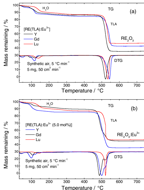
Figure 2. TG and DTG curves (a) [\text{RE}(\text{TLa})] and (b) [\text{RE}(\text{TLa})\text{:Eu}^{3+} (5.0 mol%)] ( \text{RE}^{3+} : Y, Gd and Lu).
