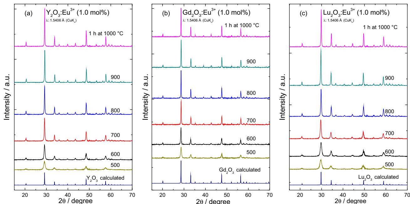
Figure 3. XPD patterns of (a) \text{Y}_2\text{O}_3\text{:Eu}^{3+} , (b) \text{Gd}_2\text{O}_3\text{:Eu}^{3+} and (c) \text{Lu}_2\text{O}_3\text{:Eu}^{3+} (1.0 mol%) materials annealed for 1 h at different temperatures; reference pattern: PDF: 86-2477 and 86-2475, respectively.
