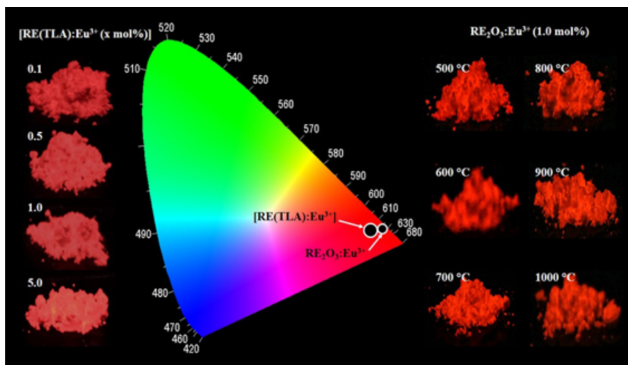
Figure 8. CIE diagram (center) and images of [\text{RE}(\text{TLA})\cdot\text{Eu}^{3+}] (left) and \text{RE}_2\text{O}_3\cdot\text{Eu}^{3+} (right), excited at 254 nm.
