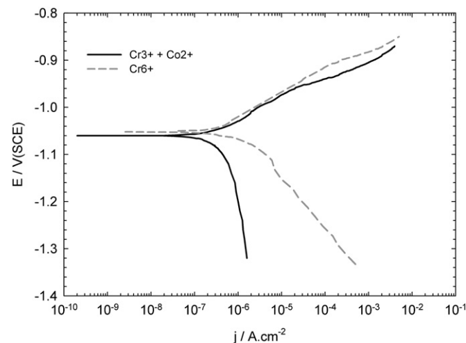
Fig. 4. Polarization curves for Cr 3+ + Co 2+ -treated or Cr 6+ -treated electrogalvanized steel samples immersed in a 0.1 mol/L Na 2 SO 4 solution.
