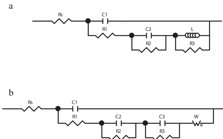
Fig. 7. Equivalent circuits used to model \text{Cr}^{3+} + \text{Co}^{2+} - or \text{Cr}^{6+} -treated samples immersed in a naturally aerated 0.1 mol/L \text{Na}_2\text{SO}_4 solution for 96 h.
