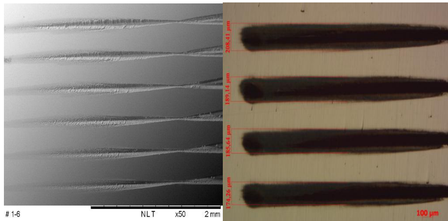
Fig. 3. In the left, SEM image showing the six more deep grooves generated by the D-Scan technique in VI 138 steel. In the right, OM image shows where 2\rho_{\max} where measured.
