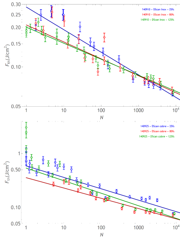
Fig. 4. Ablation thresholds ( F_{th} ) X number of overlapping pulses ( N ) for stainless steel VI 138 (up) and copper (down).
