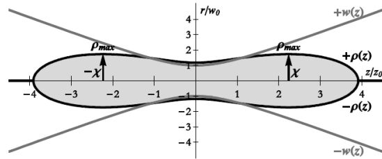
Fig. 1. Profile recorded on the sample surface having two lobes at maximum transverse position X with the maximum dimension 2\rho_{\text{max}} . Lines +W(z) and -W(z) represents the profile of the laser beam where the intensity is 1/e^2 of the peak value.
