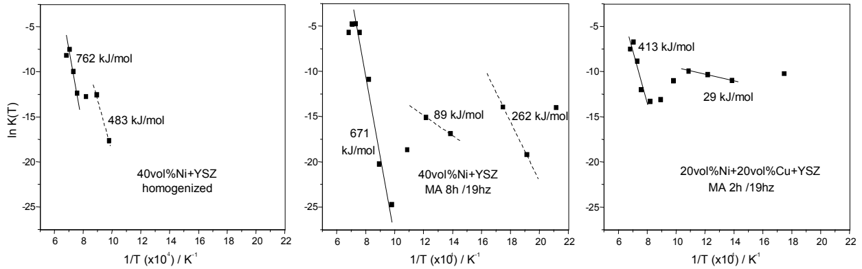
Fig. 9. Activation energies determined by SID method for homogenized and MA powder pellets up to 1200°C; polymer vials.
