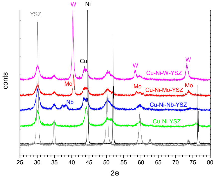
Fig. 6. X-ray profiles for 8vol% Me- 12vol% Cu- 20vol% Ni – YSZ; Me = W, Nb, Mo.
