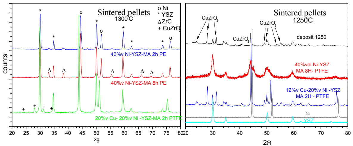
Fig. 7. X-ray analysis of sintered MA powders under argon, milled in polymer vials.
