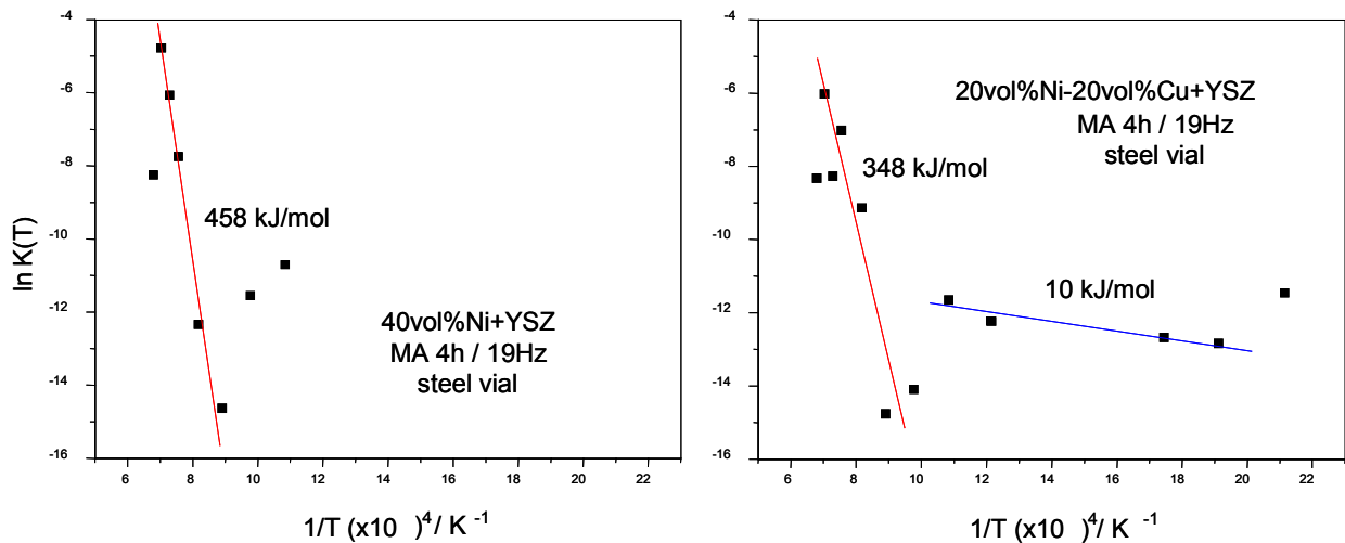
Fig. 10. Activation energies; steel vials.
