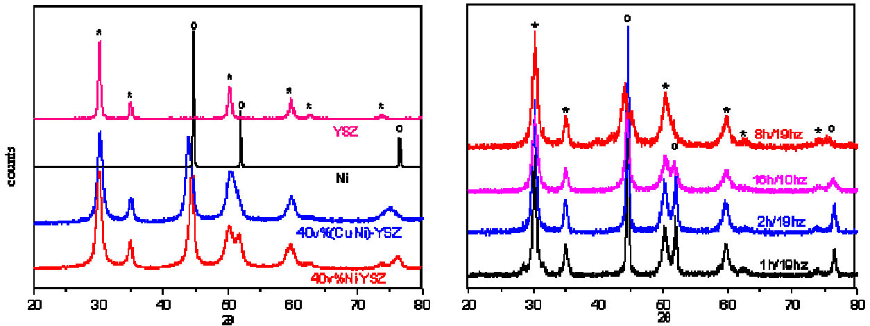
Fig. 4. X-ray profiles of MA powders (Cu-)Ni-YSZ; ° Ni ; * YSZ
