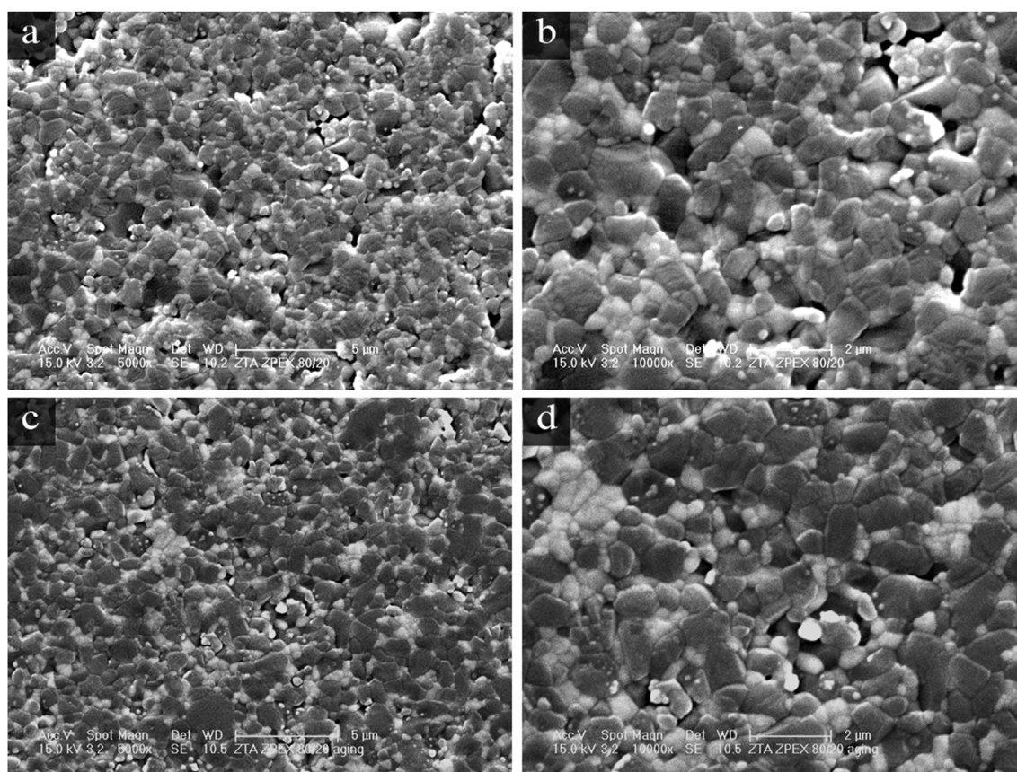
Fig. 6. SEM micrographs of the ZTA composite surface before aging (a, 5,000x; b, 10,000x), and after aging protocol (c, 5,000x; d, 10,000x). The images demonstrate the microstructural arrangement and final density obtained for the ZTA composite, where a few defects related to ceramic processing can be observed. In addition, the established aging protocol did not cause evident microstructural changes.
