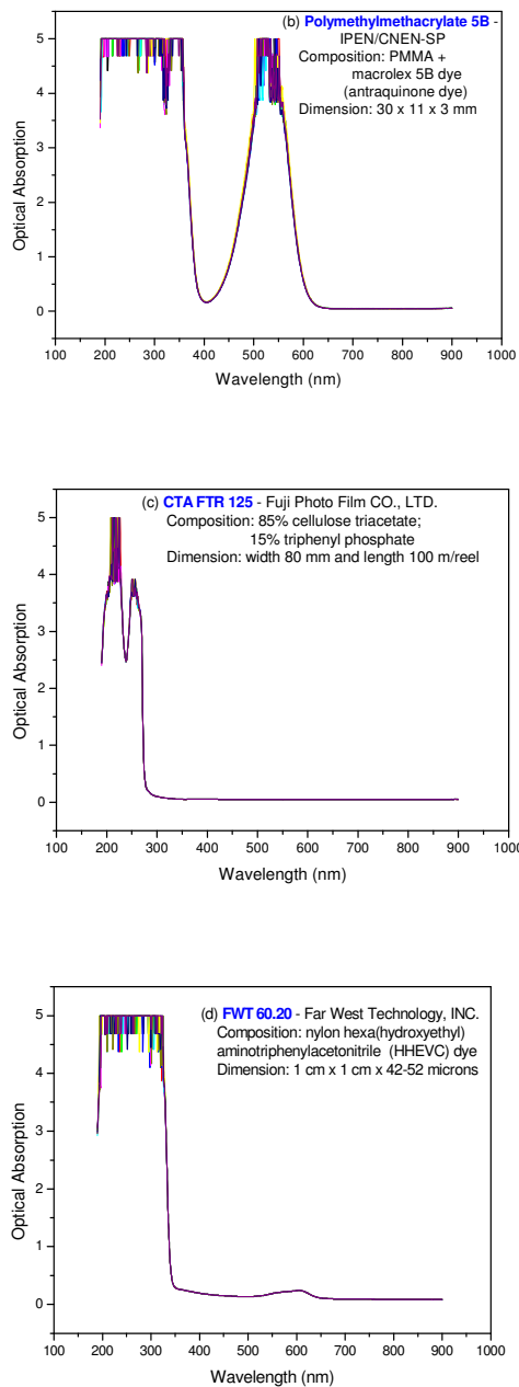
Figure 1. Optical absorption spectra of non-irradiated radiochromic films.
