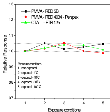
Figure 2. Temperature effect on PMMA Red 5B, PMMA Red 4034 and CTA samples at range between 4°C and 100°C.
