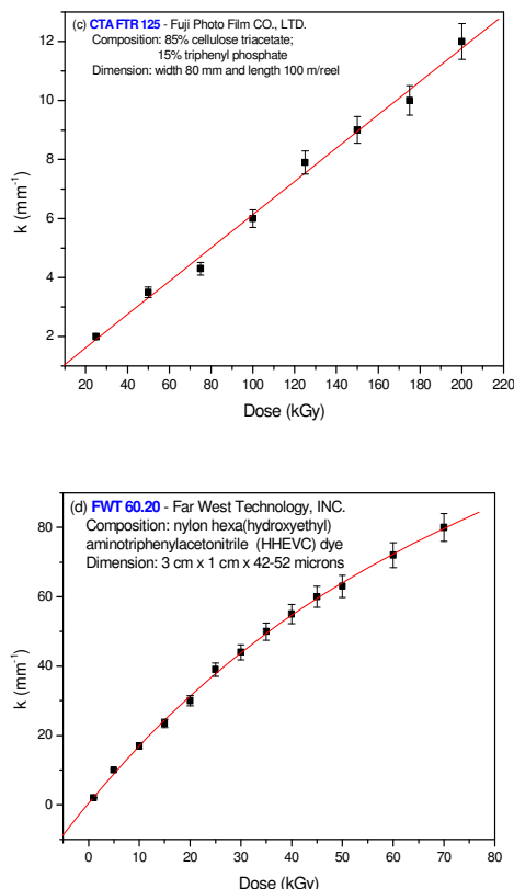
Figure 4. Dose response calibration curves of PMMA Red 5B, PMMA Red 4034, CTA FTR-125 and FWT 60.20 films.
