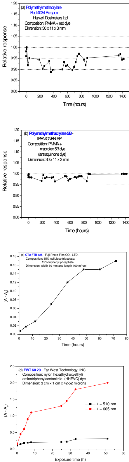
Figure 3. Ambient light influence on Red 4034, Red 5B, CTA and FWT film.
