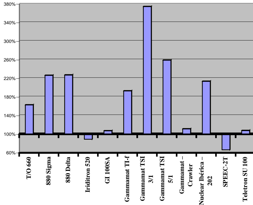
Figure 1 - Efficiency of the projectors in relation to exposition rate.
