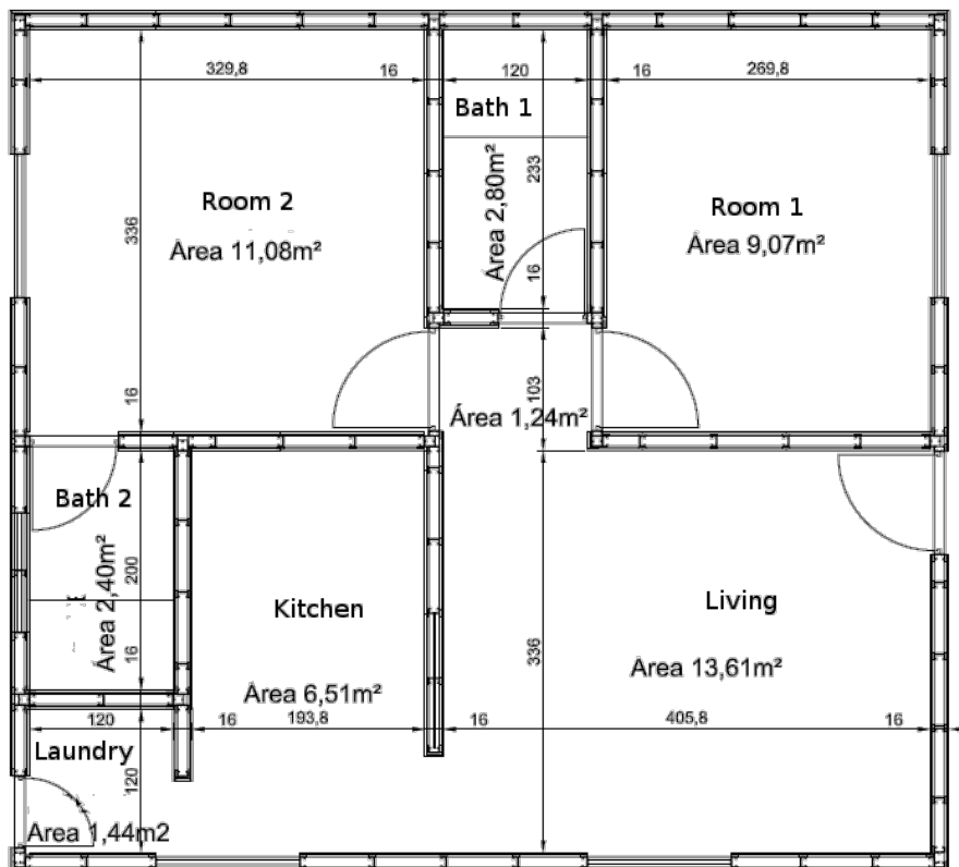
Figure 19: Floor plan of the experimental house built with gypsum boards [27]
