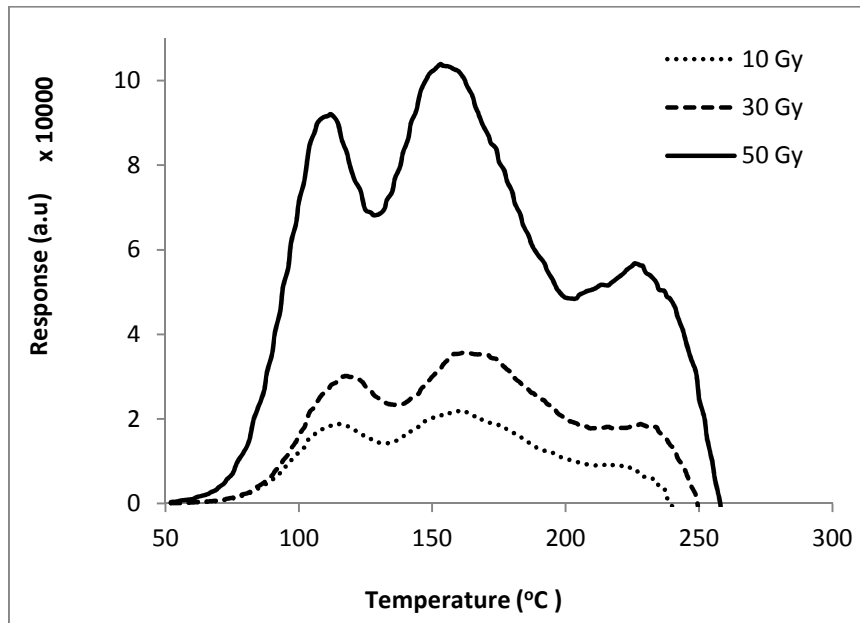
Figure. 1 Glow curve of topaz: glass composite in ratio 2:1, sintered at 1000 °C for one hour, irradiated for the various doses with Beta irradiator and TL read out with Harshaw (TLD-3500) at the heating rate of 5 °C/s.
