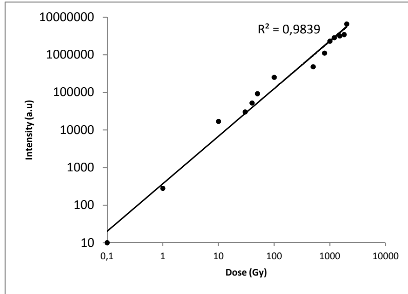
Figure. 3. Intensity of Peak 1 of topaz composites irradiated for the various doses with Beta irradiator and TL read out with Harshaw (TLD-3500) at the heating rate 5^\circ\text{C/s} .
