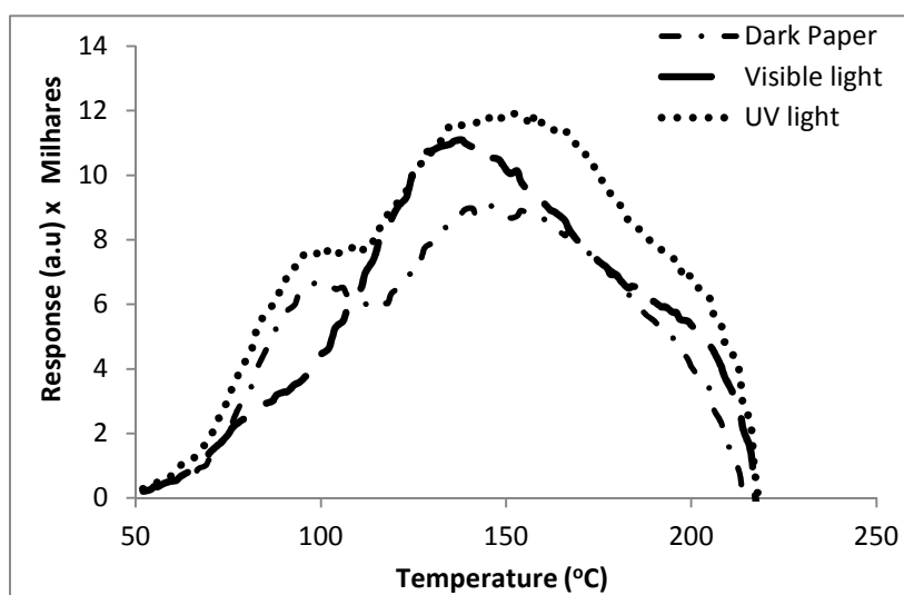
Figure 5. Effect of visible and UV light on the topaz glass composite irradiated with dose about 15 Gy with Beta irradiator and TL read out with Harshaw (TLD-3500) at the heating rate of 5°C/s under different environmental condition.
