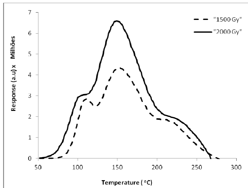
Figure. 2 Glow curve of topaz: glass composite in ratio 2:1, sintered at 1000 °C for one hour, irradiated for 1500 and 2000 Gy doses with Beta irradiator and TL read out with Harshaw (TLD-3500) at the heating rate of 5 °C/s.
