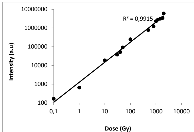
Figure. 4. Intensity of Peak 2 of topaz composites irradiated for the various doses with Beta irradiator and TL read out with Harshaw (TLD-3500) at the heating rate 5^\circ\text{C/s} .
