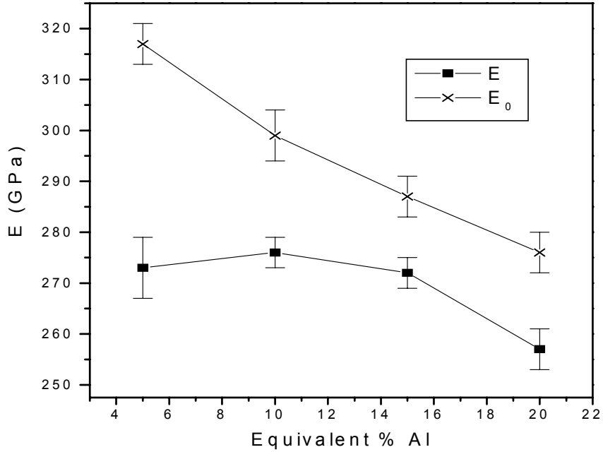
Figure 1 – Elastic modulus (E and E 0 ) with variation of the aluminum concentration for samples pressure-less sintered.
