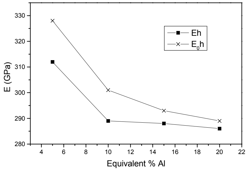
Figure 2 - Elastic modulus (E and E 0 ) with variation of the aluminum concentration for samples sintered and subsequently subjected to HIP.
