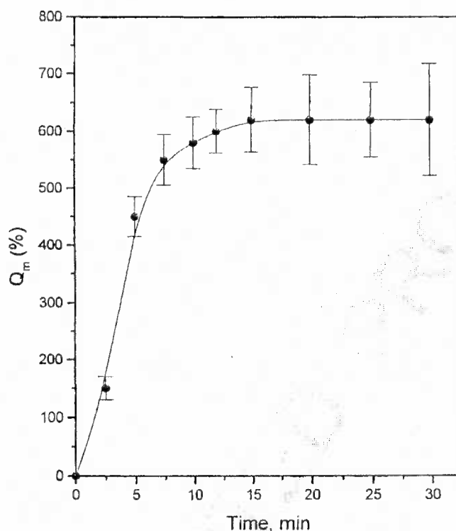
Swelling degree ( Q_{max} ) of PGLD-ChB dendrimer measured by ATR-FT-IR after integration of the water absorption band.
