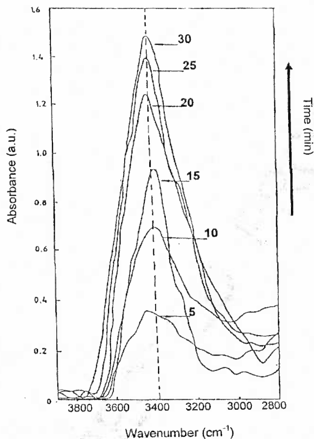
ATR-FT-IR spectra of PGLD-ChB dendrimer exposed to water for different intervals of time.
