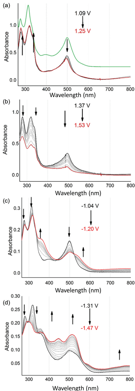
Figure 2. (a) Electronic spectrum of [\text{Ru}(\text{TPAtpy})(\text{ctpy})](\text{PF}_6)_3 (green line), and spectroelectrochemical changes associated with the first oxidation (a), second oxidation (b), first reduction (c) and second reduction (d), both in DMF solution.
