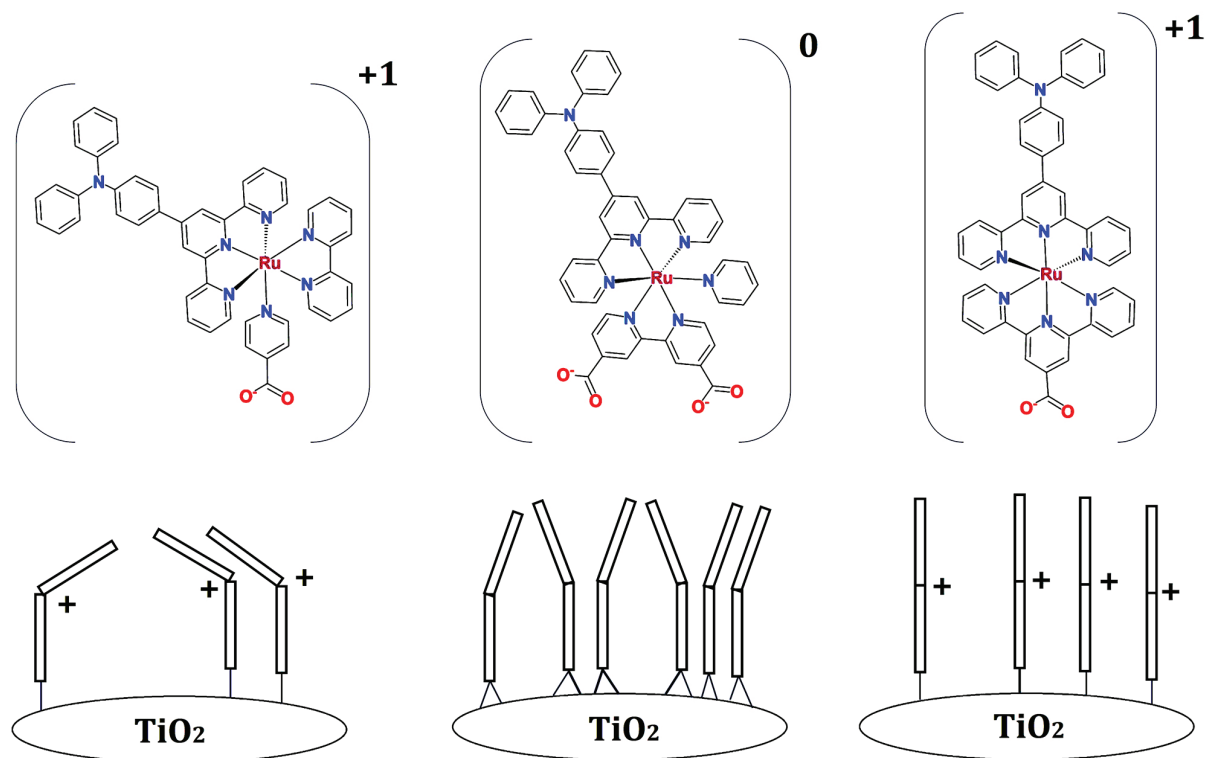
Scheme 1. Scheme showing the influence of the ruthenium dye molecular structure on the surface concentration and charge on the \text{TiO}_2 mesoporous film.
