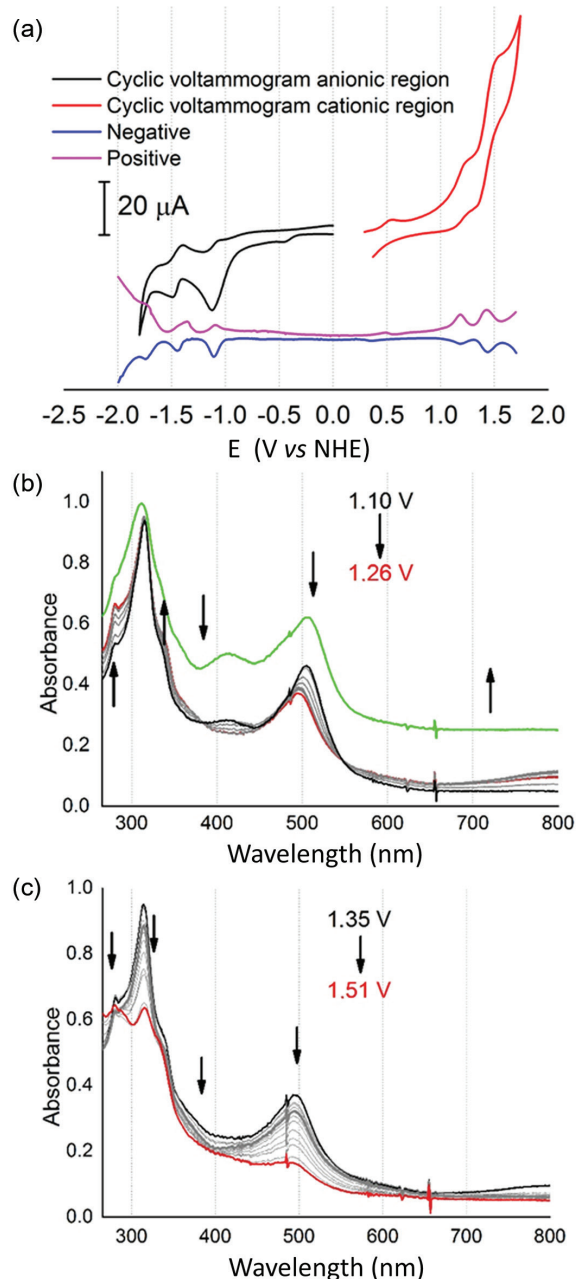
Figure 5. (a) Cyclic voltammogram of 1.0 mM [\text{Ru}(\text{py})(\text{dcbpy})(\text{TPAtpy})] in 0.10 M \text{TBAClO}_4 DMF solution as electrolyte, \nu = 100 \text{ mV s}^{-1} , (b) electronic spectrum of [\text{Ru}(\text{py})(\text{dcbpy})(\text{TPAtpy})] (green line) and spectroelectrochemical behavior associated with the first and (c) second oxidation processes.
