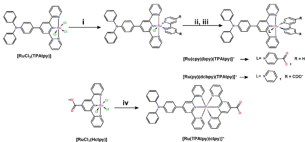
Scheme 2. Scheme depicting the strategy used to prepare the [Ru(TPATpy)(ctpy)](PF_6)_2 , [Ru(py)(dcbpy)(TPATpy)] and [Ru(cpy)(bpy)(TPATpy)](PF_6)_2 push-pull ruthenium dyes. (i) LiCl, bpy (or dcbpy) in 3:1 v/v ethanol:water mixture, refluxed for 4 h, followed by addition of NH_4PF_6(aq) . (ii) AgNO 3 in acetone:water (3:5) v/v mixture, refluxed for 4 h. Filtered on a celite bed and removed on a rotary evaporator. (iii) Pyridine (or isonicotinic acid) in EtOH:water (1:1) v/v mixture, refluxed for 24 h, NH_4PF_6(aq) . (iv) TPAtpy ligand, MeOH:H 2 O (5:1) mixture, refluxed for 12 h, NH_4PF_6(aq) .
