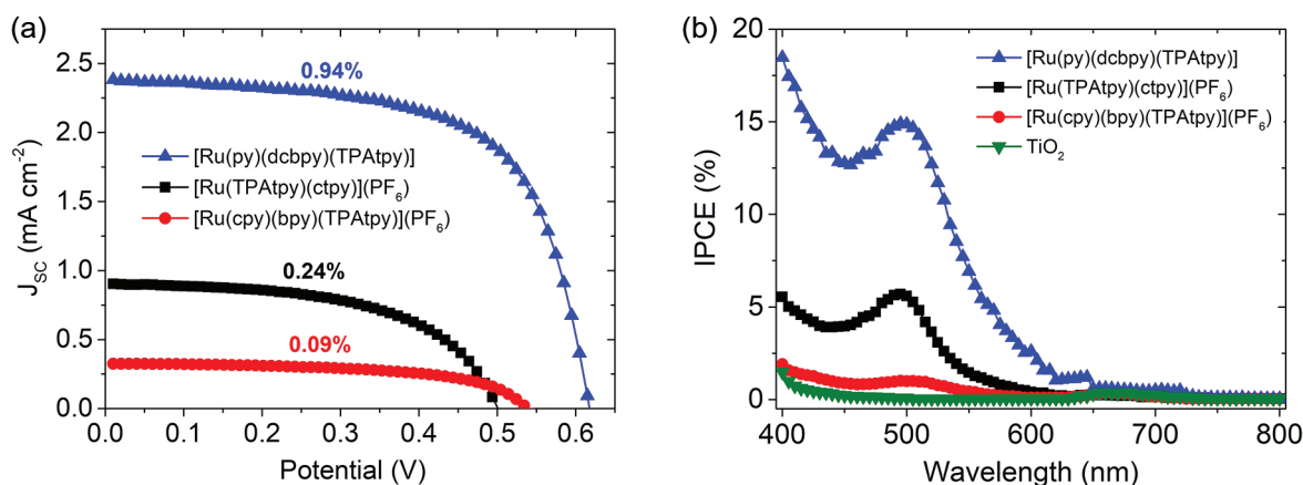
Figure 7. (a) JV curves with their respective overall photoconversion efficiencies, and (b) the IPCE curves DSSCs prepared with the [\text{Ru}(\text{py})(\text{dcbpy})(\text{TPAtpy})] , [\text{Ru}(\text{TPAtpy})(\text{ctpy})](\text{PF}_6) and [\text{Ru}(\text{cpy})(\text{bpy})(\text{TPAtpy})](\text{PF}_6) push-pull ruthenium dyes.
