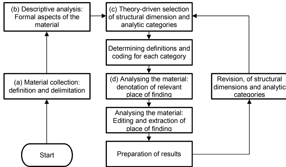
Figure 1: Research process of a structuring content analysis [6].
