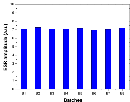
Figure 5. Reproducibility of the dosimeter production process to an absorbed dose of 2 Gy.
