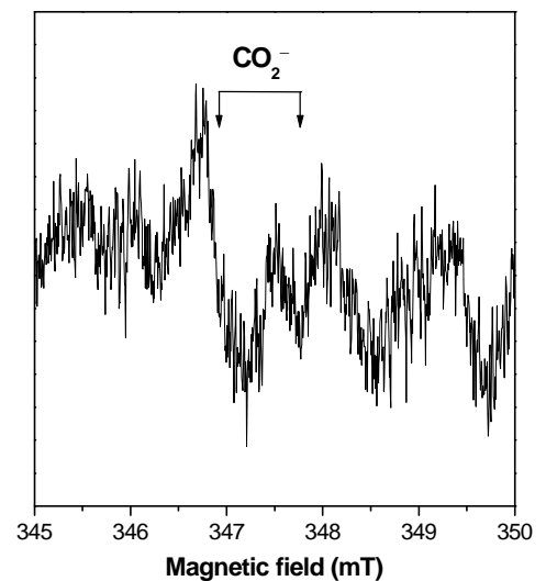
Figure 4. A-type apatite ESR spectrum irradiated to an absorbed dose of 0.2 Gy.
