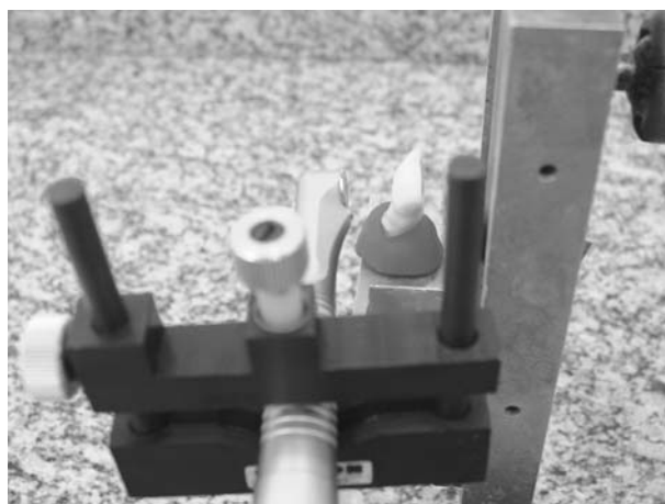
FIG. 2. Sample positioned on a metallic support, as well as the laser handpiece.
