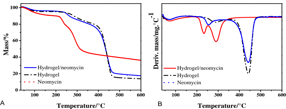
Fig. 4: (A) TG and (B) DTG curves for non-irradiated neomycin, hydrogel/neomycin and hydrogel, obtained under N 2 flow.
