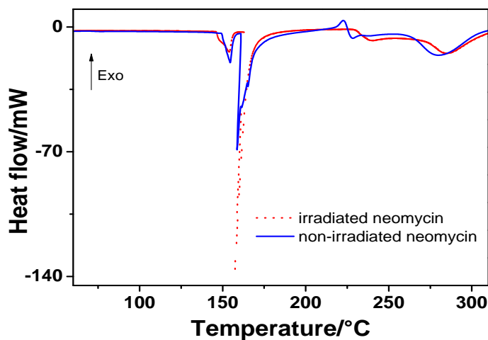
Fig. 3: DSC profiles of neomycin irradiated and non-irradiated.
