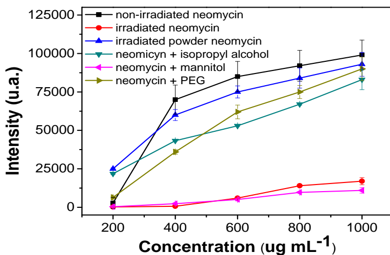
Fig. 2: Neomycin stability irradiated of at 25kGy. Comparison between different radioprotectors.
