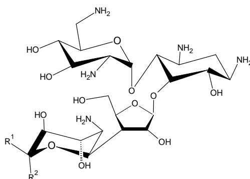
Fig. 1: Neomycin chemical structure; R1= CH 2 NH 2 ; R2 =H 2 .
