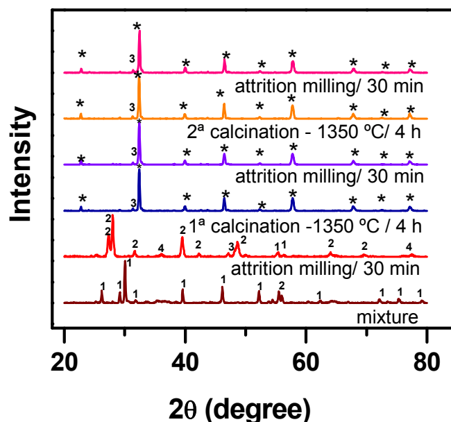
Fig. 6: X-ray diffraction patterns of powder mixtures after each processing step of route R2. 1- \text{La}_2\text{O}_3 , 2- \text{La}(\text{OH})_3 3- \text{SrLaGaO}_4 , 4- \text{Ga}_2\text{O}_3 e * - LSGM.
