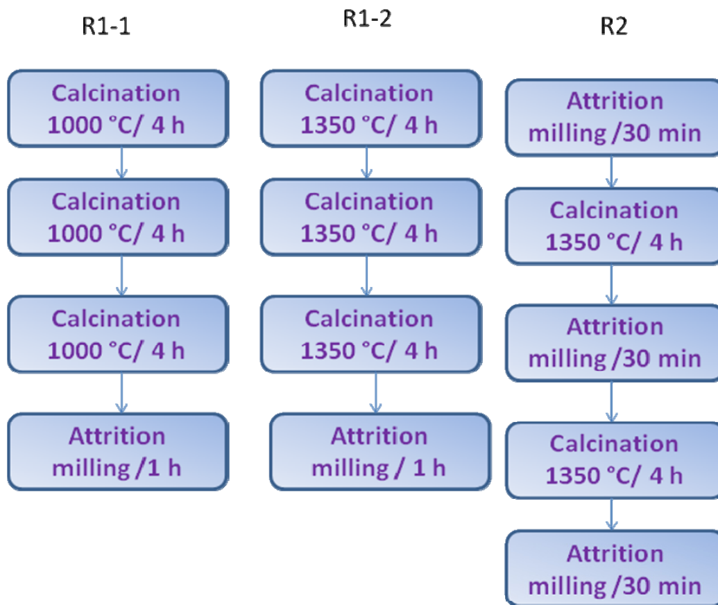
Fig. 1: Flowchart of the processing routes.
