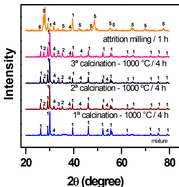
Fig. 2: X-ray diffraction patterns of powder mixtures after each processing step of route R1-1. 1-La 2 O 3 , 2-SrCO 3 , 3-SrLaGaO 4 , 4-Ga 2 O 3 , 5-La(OH) 3 e 6-La 4 Ga 2 O 9 .
