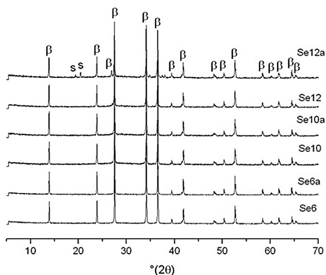
Figure 1: X-ray powder diffraction of the sintered samples ( \beta is \beta - \text{Si}_3\text{N}_4 and s is \text{Si}_2\text{ON}_2 ).
