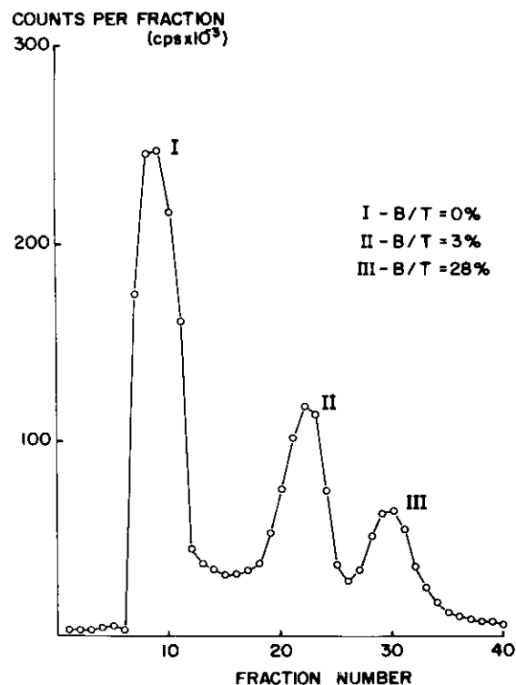
Figure 1. Elution profile of a CM-Sephadex C-25 chromatography of the iodinated products obtained after Chloramint T radioiodination of hPTH (1-34). B/T indicate the percent binding of the iodinated product obtained under normal assay condition.
