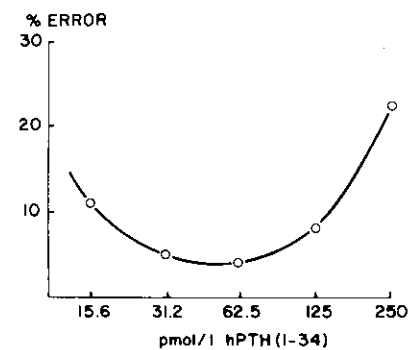
Figure 3. Precision profile obtained with a typical hPTH (1-34) assay using standard assay conditions.
